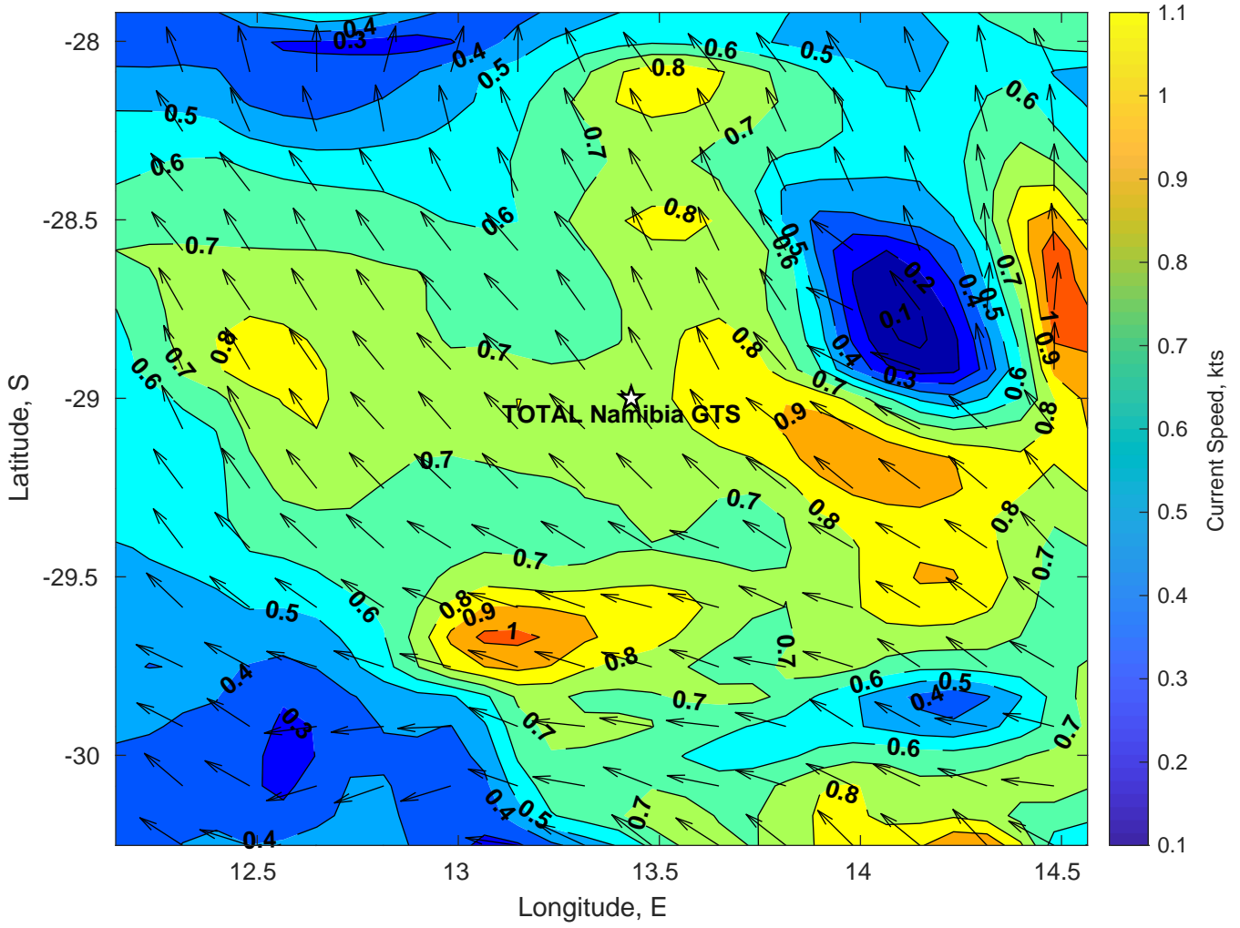
Surface Currents for TOTAL Namibia GTS at 02-Mar-2025 00:00:00
