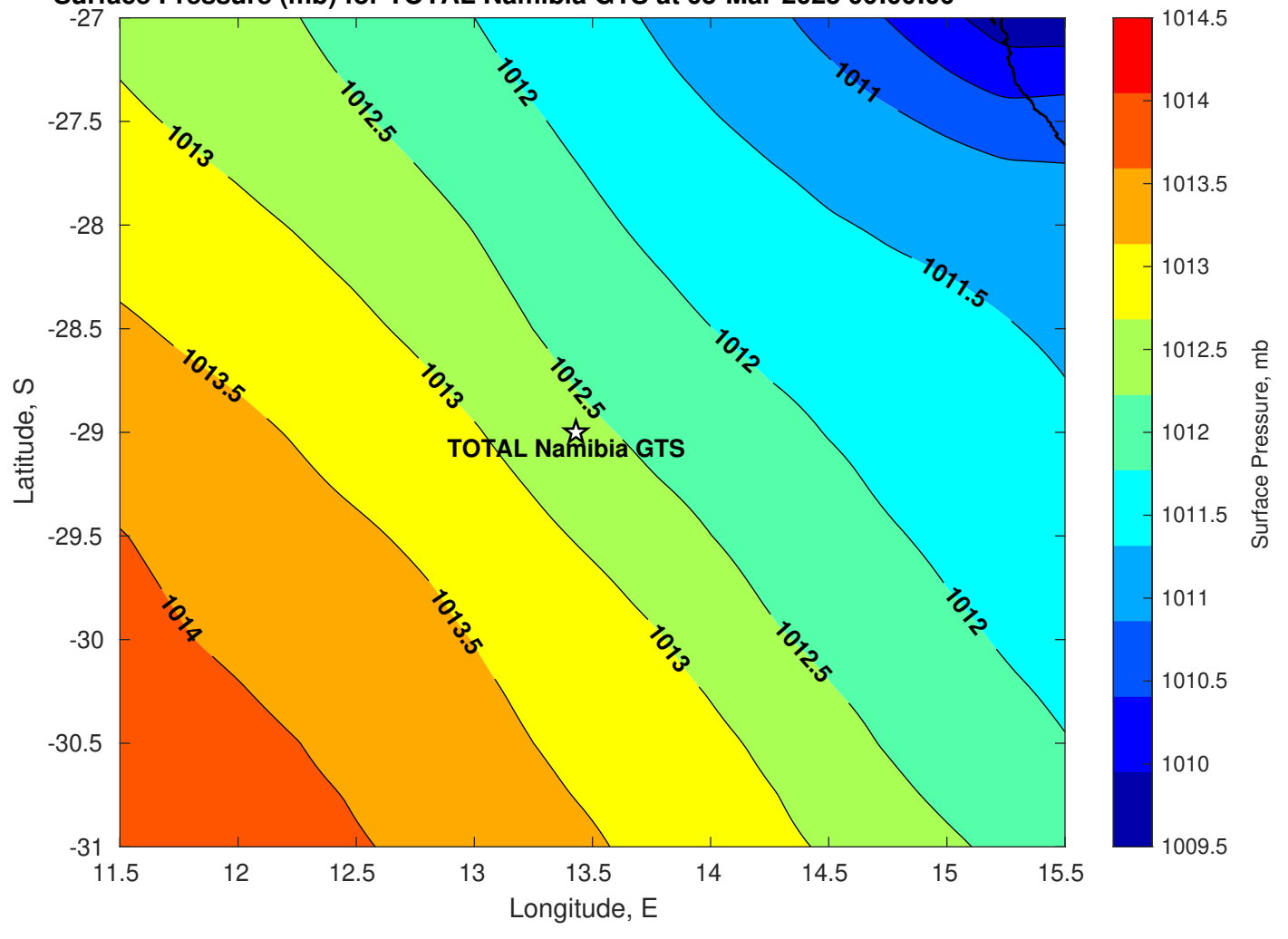
Surface Pressure (mb) for TOTAL Namibia GTS at 05-Mar-2025 00:00:00
