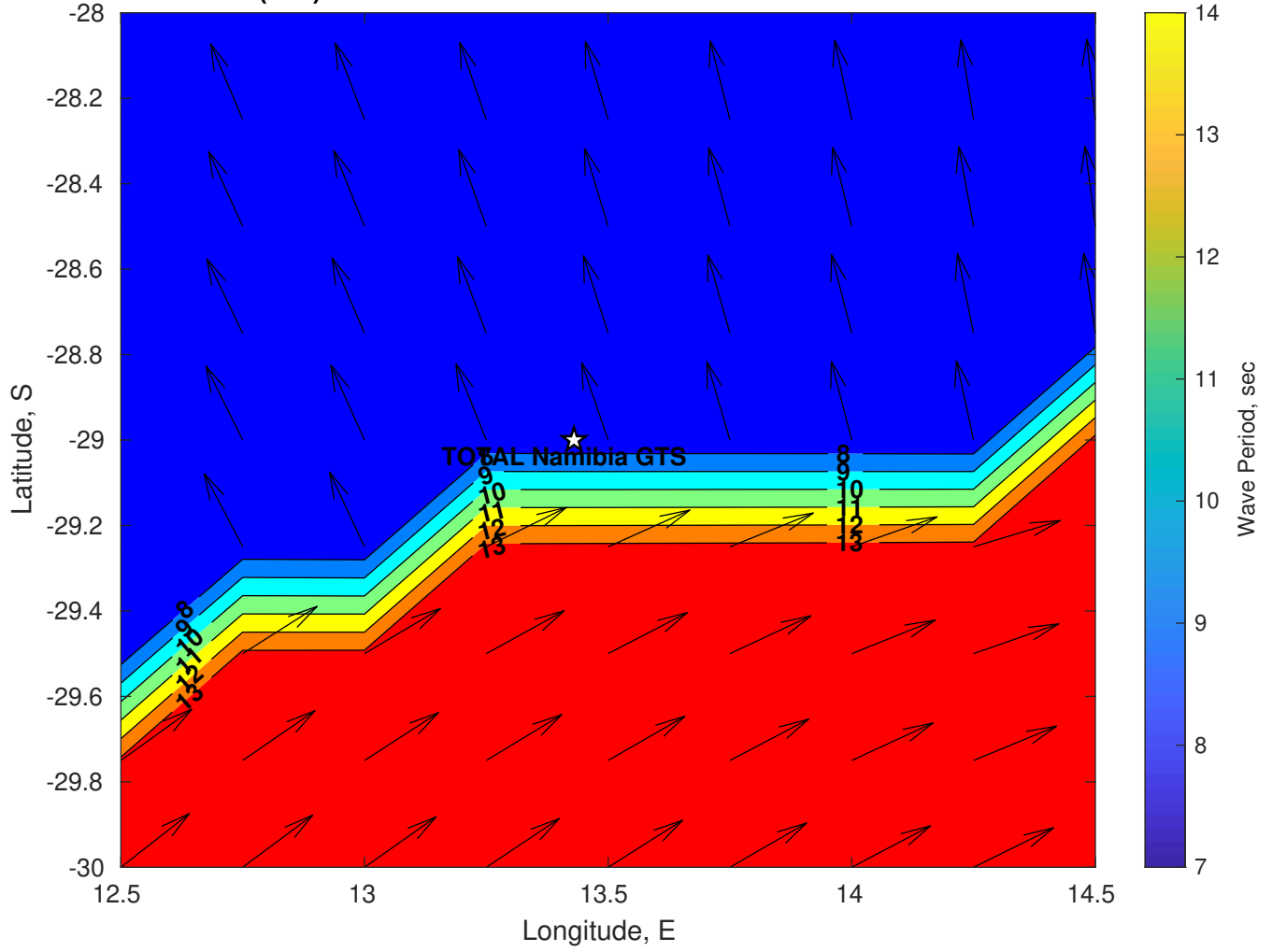
Wave Period (sec) for TOTAL Namibia GTS at 03-Mar-2025 09:00:00
