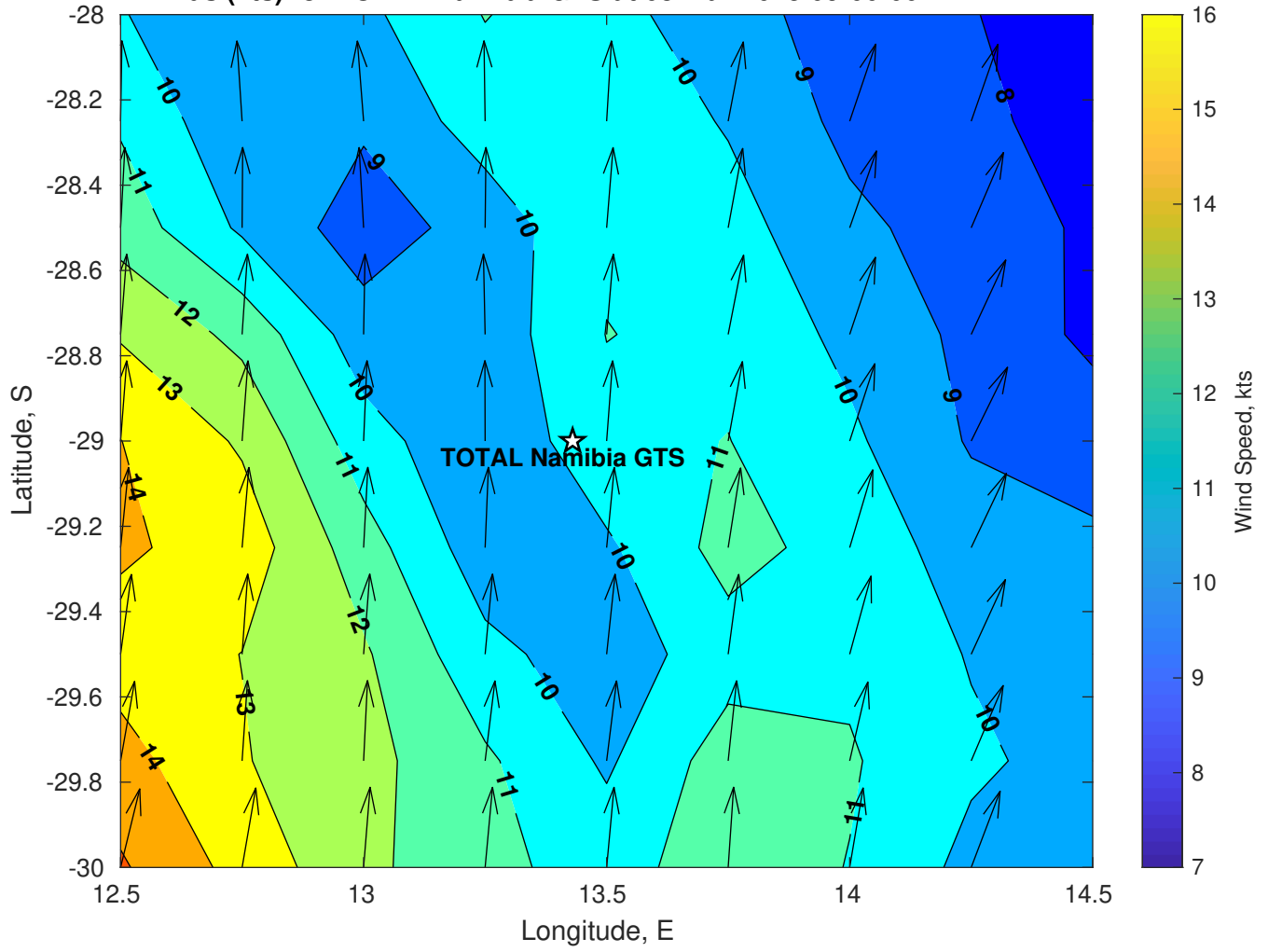
Winds (kts) for TOTAL Namibia GTS at 03-Mar-2025 09:00:00
