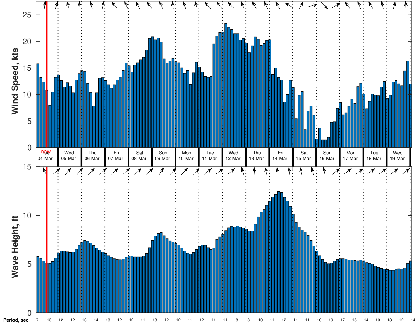
Wind & Wave Forecast for TOTAL Namibia GTS from 03-Mar-2025 02:00:00 to 19-Mar-2025 02:00:00
