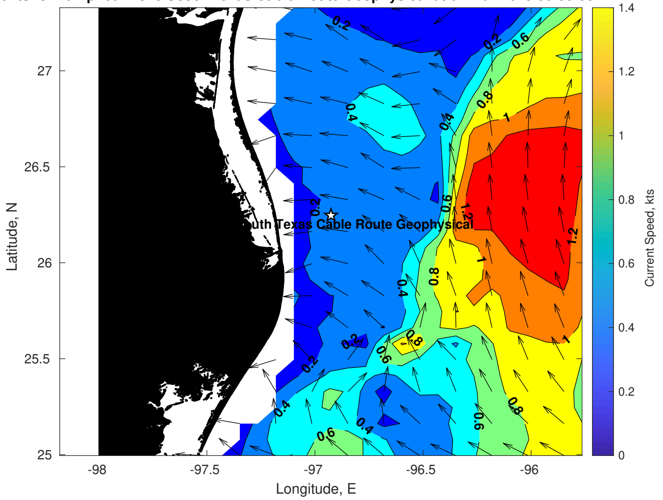
Surface Currents for Tampnet P2378 South Texas Cable Route Geophysical at 02-Mar-2025 00:00:00
