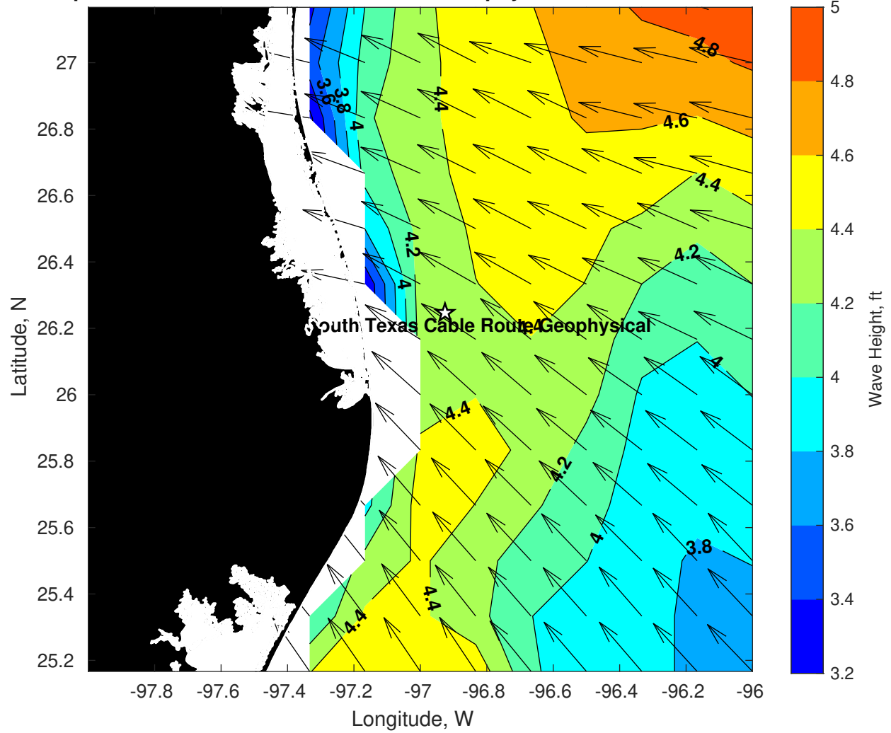
Wave Height (ft) for Tampnet P2378 South Texas Cable Route Geophysical at 03-Mar-2025 09:00:00
