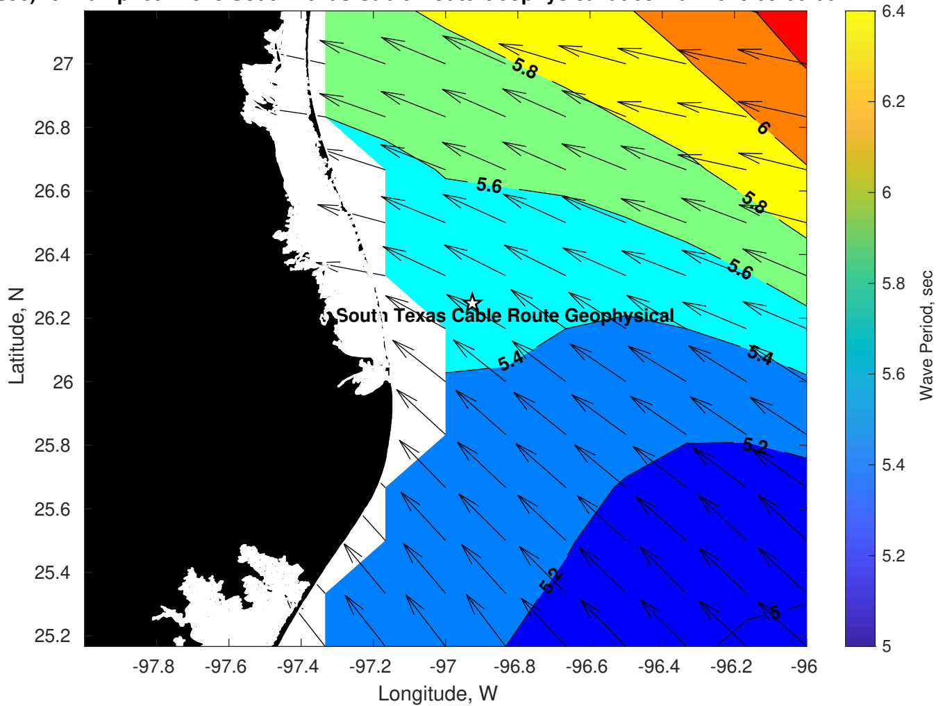
Period (sec) for Tampnet P2378 South Texas Cable Route Geophysical at 03-Mar-2025 09:00:00
