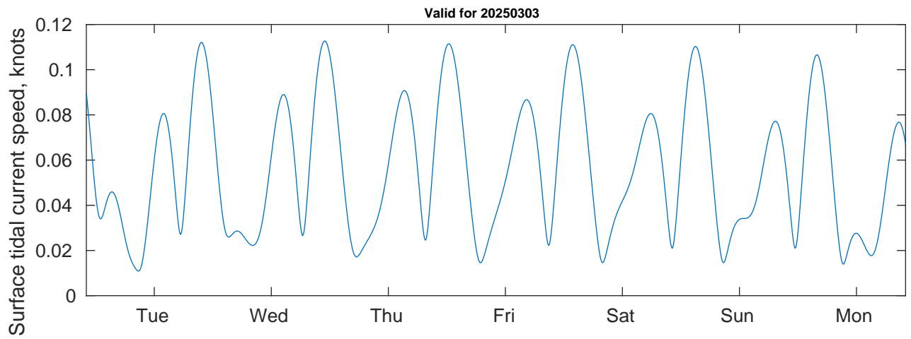
Tidal Currents and Heights for Tampnet P2378 South Texas Cable Route Geophysical at 20250303
