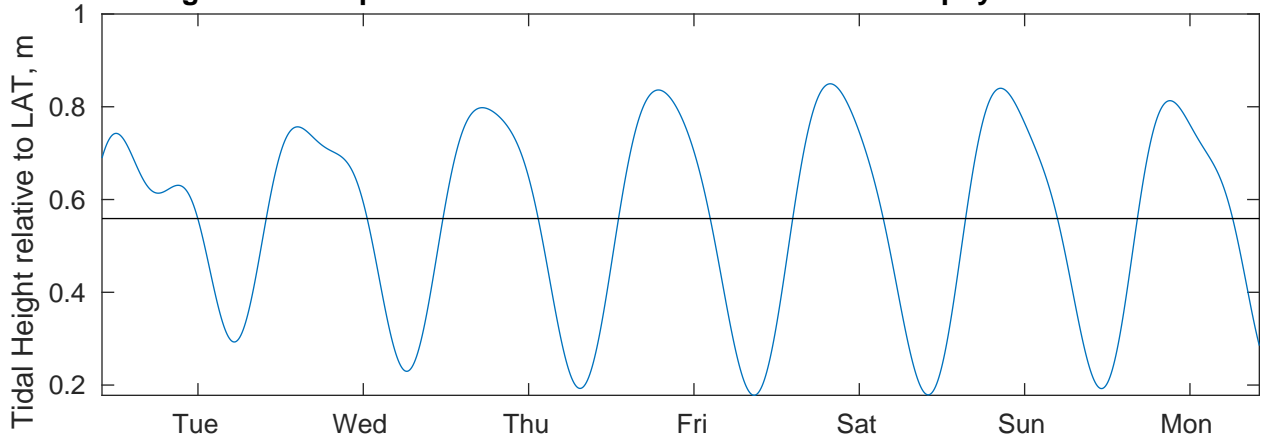
Tidal Currents and Heights for Tampnet P2378 South Texas Cable Route Geophysical at 20250303
