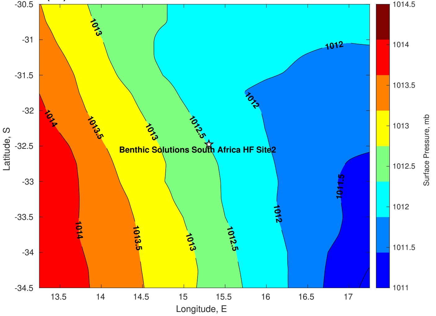
Surface Pressure (mb) for Benthic Solutions South Africa HF Site2 at 04-Mar-2025 00:00:00
