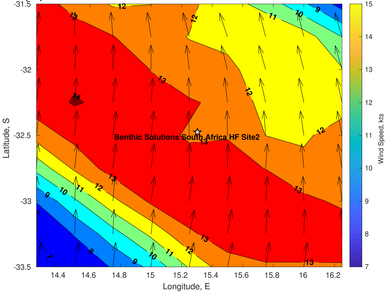
Winds (kts) for Benthic Solutions South Africa HF Site2 at 04-Mar-2025 09:00:00
