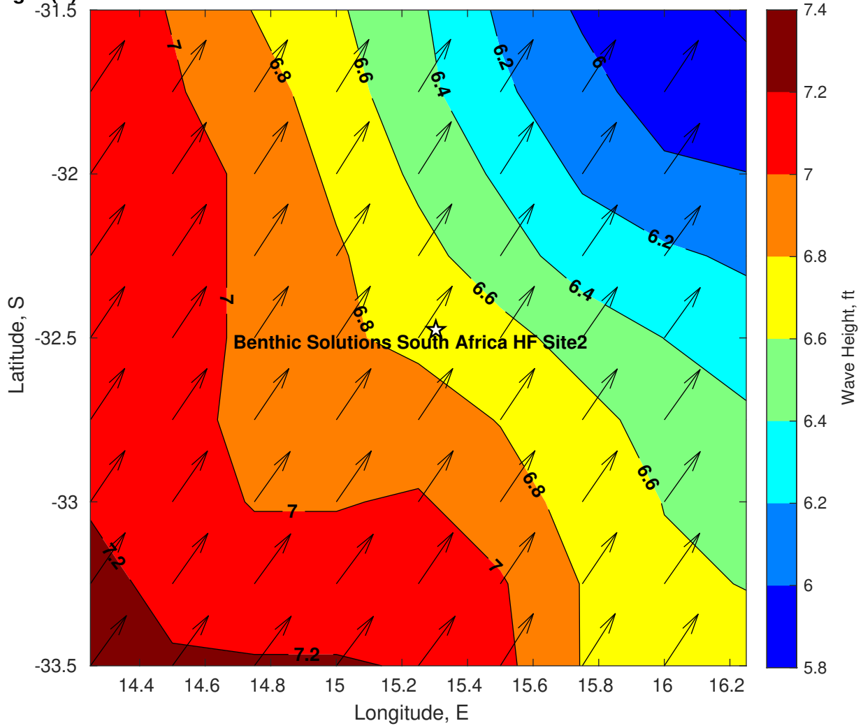
Wave Height (ft) for Benthic Solutions South Africa HF Site2 at 04-Mar-2025 09:00:00
