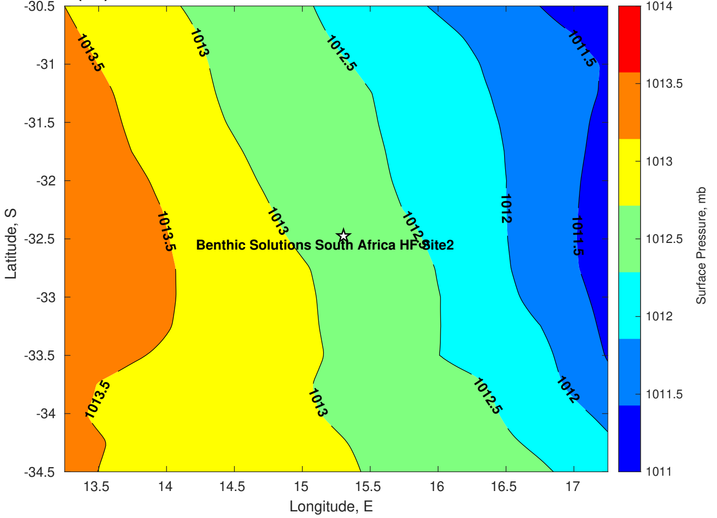
Surface Pressure (mb) for Benthic Solutions South Africa HF Site2 at 05-Mar-2025 00:00:00
