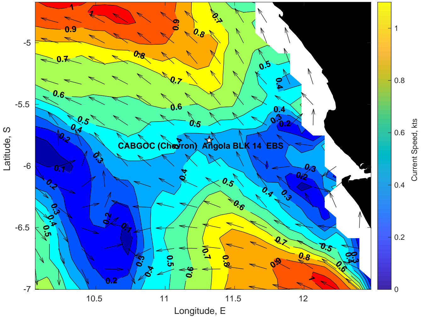
Surface Currents for CABGOC (Chevron) Angola BLK 14 EBS at 03-Mar-2025 00:00:00
