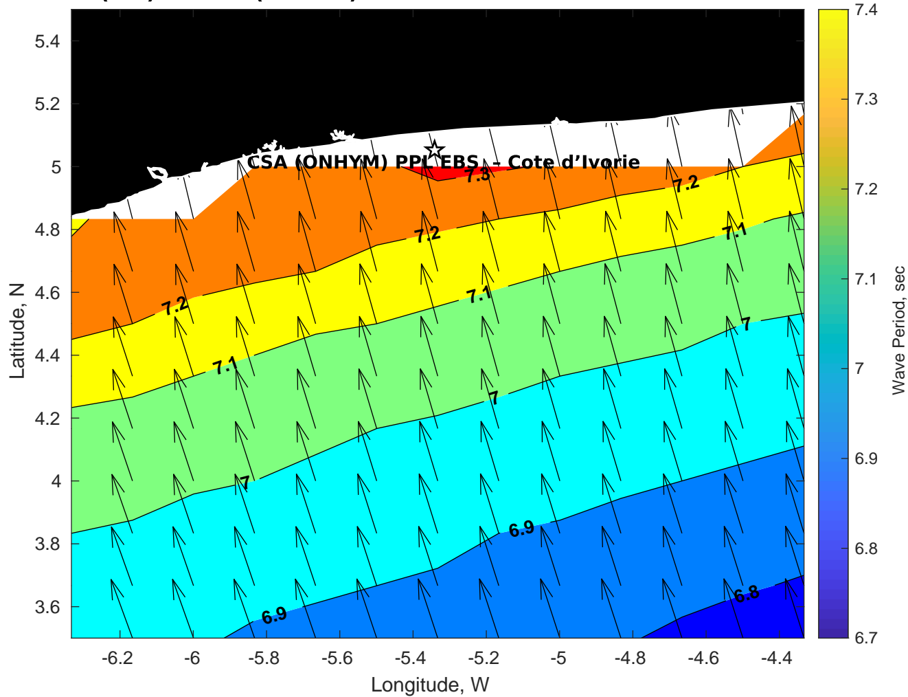
Wave Period (sec) for CSA (ONHYM) PPL EBS - Cote d'Ivoire at 04-Mar-2025 09:00:00
