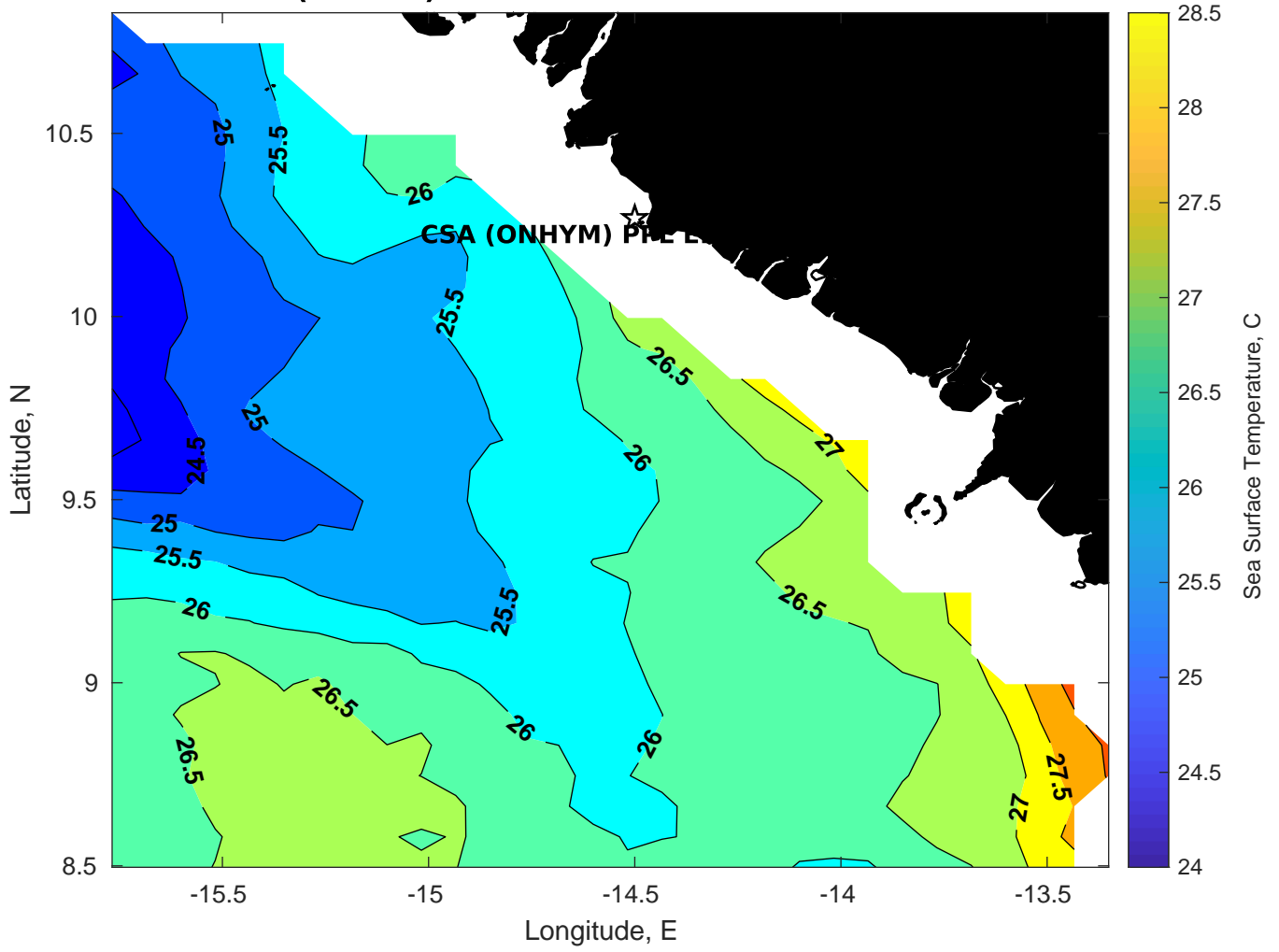
SST for CSA (ONHYM) PPL EBS - Guinea at 03-Mar-2025 00:00:00
