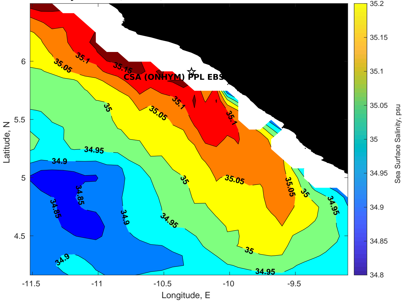
Surface Salinity for CSA (ONHYM) PPL EBS - Liberia at 03-Mar-2025 00:00:00
