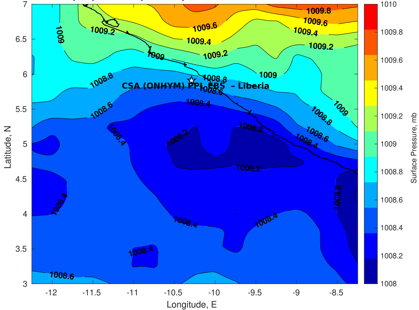
Surface Pressure (mb) for CSA (ONHYM) PPL EBS - Liberia at 05-Mar-2025 06:00:00
