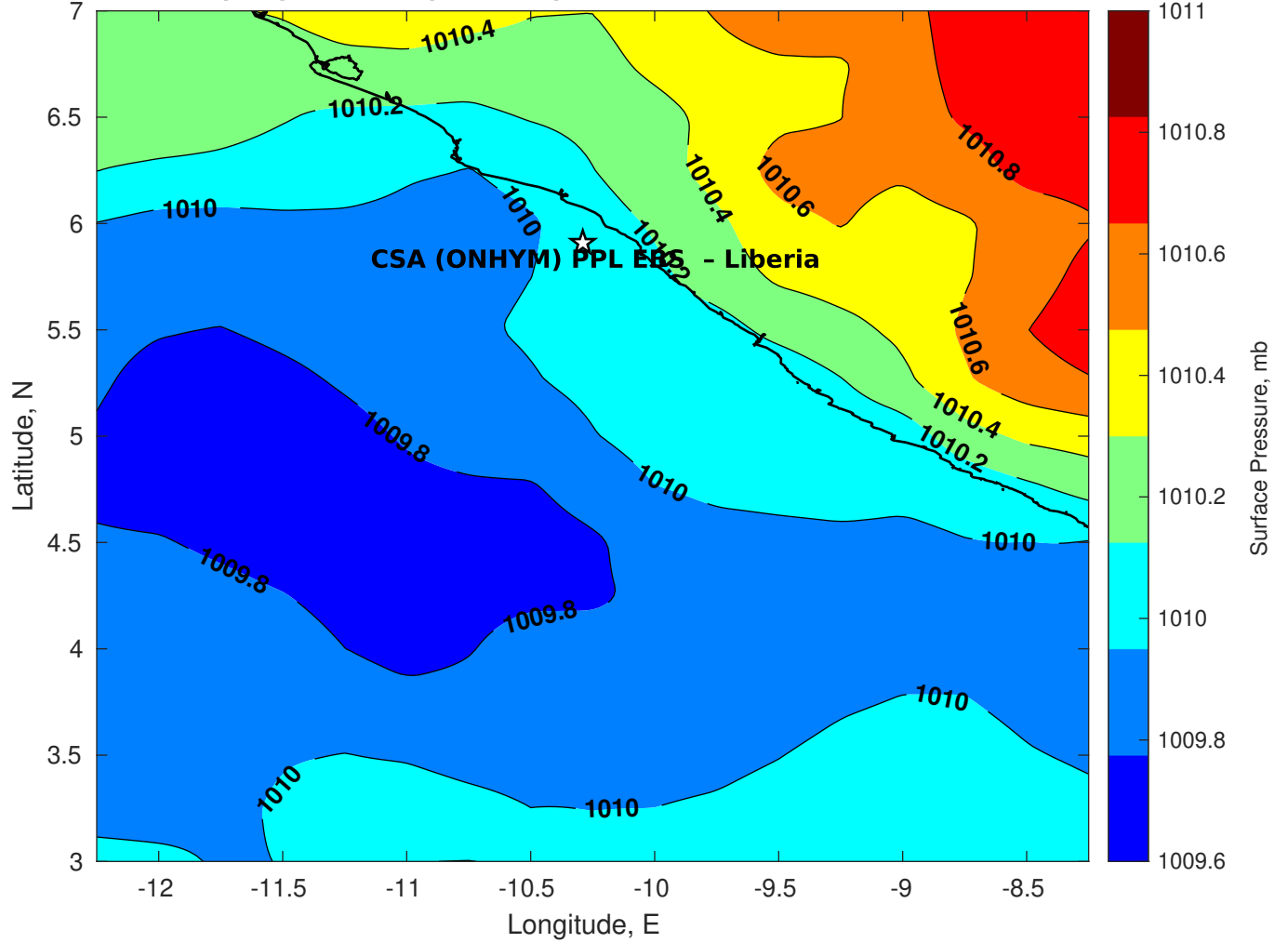
Surface Pressure (mb) for CSA (ONHYM) PPL EBS - Liberia at 06-Mar-2025 06:00:00
