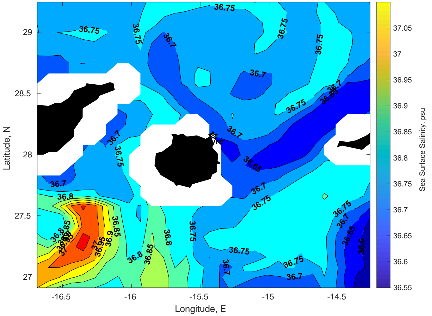
Surface Salinity for Gyre at 03-Mar-2025 00:00:00
