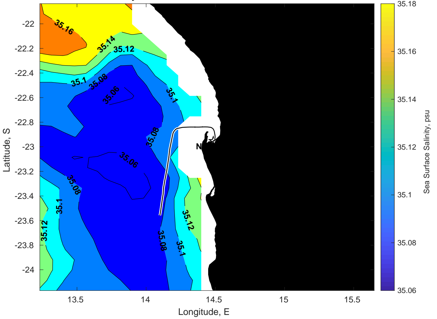
Surface Salinity for Nautilus at 03-Mar-2025 00:00:00
