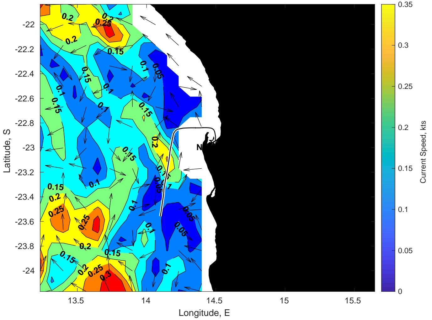
Surface Currents for Nautilus at 03-Mar-2025 00:00:00
