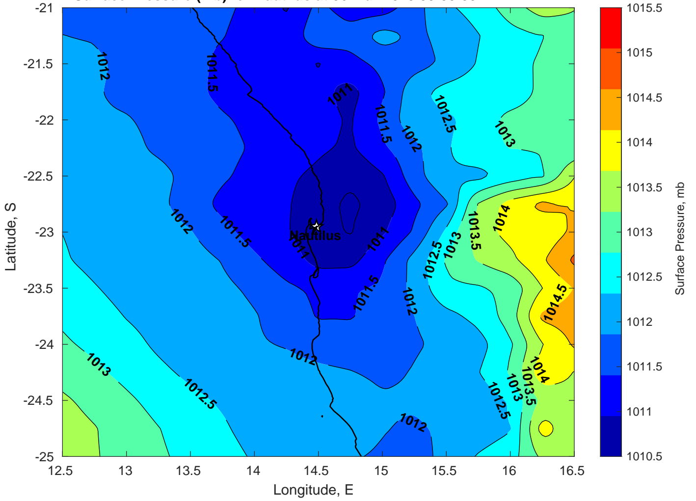
Surface Pressure (mb) for Nautilus at 06-Mar-2025 00:00:00
