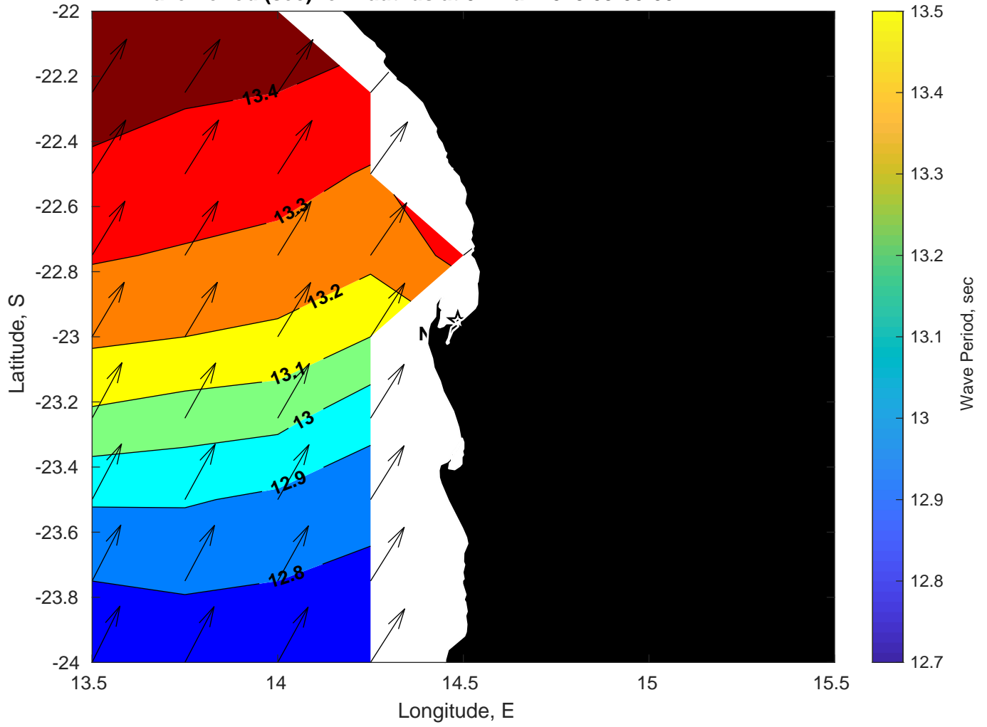
Wave Period (sec) for Nautilus at 04-Mar-2025 09:00:00
