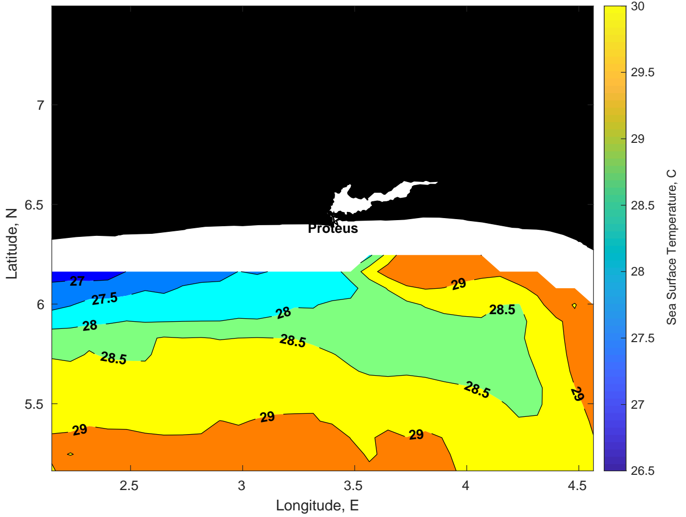
SST for Proteus at 03-Mar-2025 00:00:00
