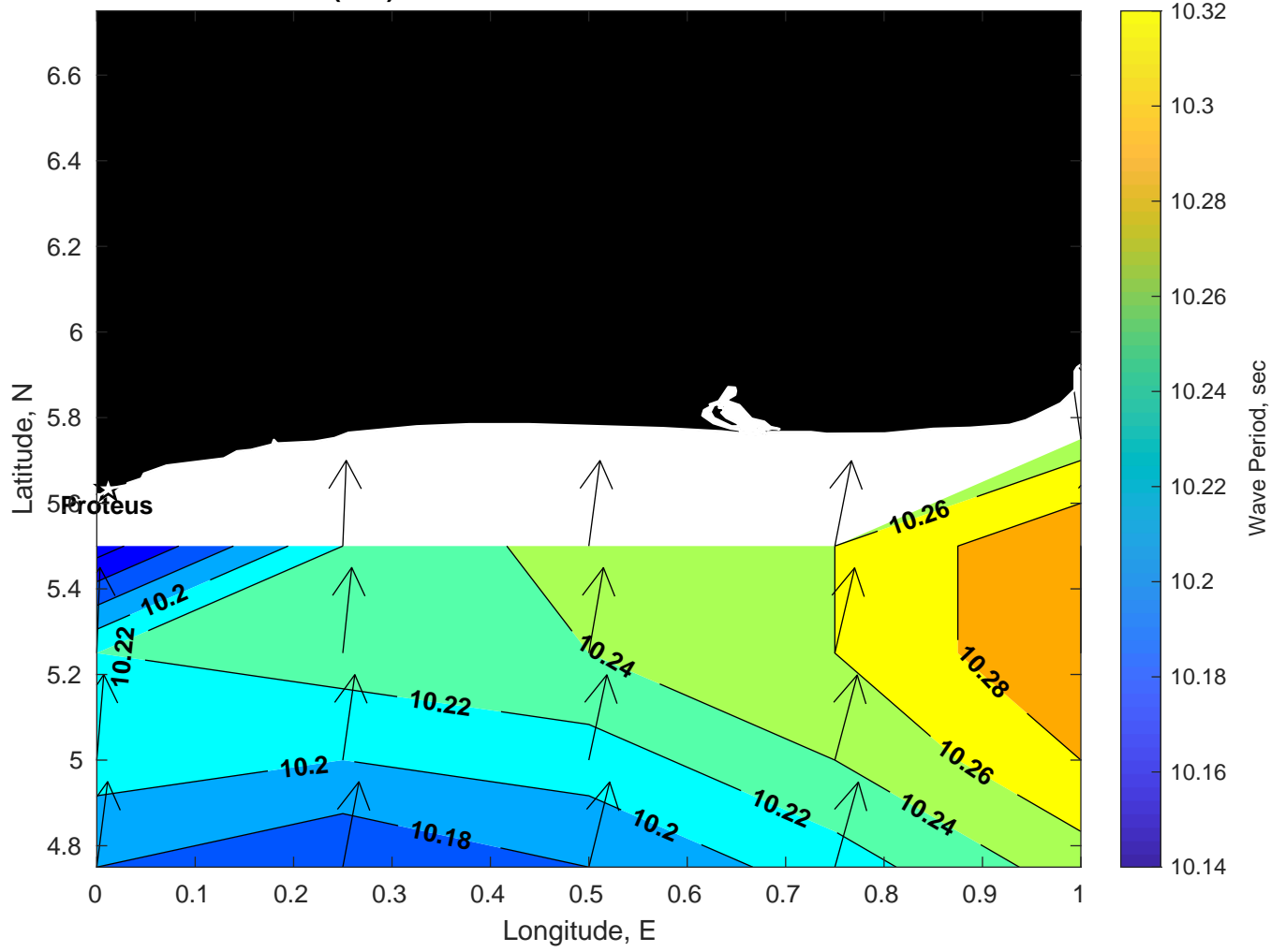
Wave Period (sec) for Proteus at 04-Mar-2025 09:00:00
