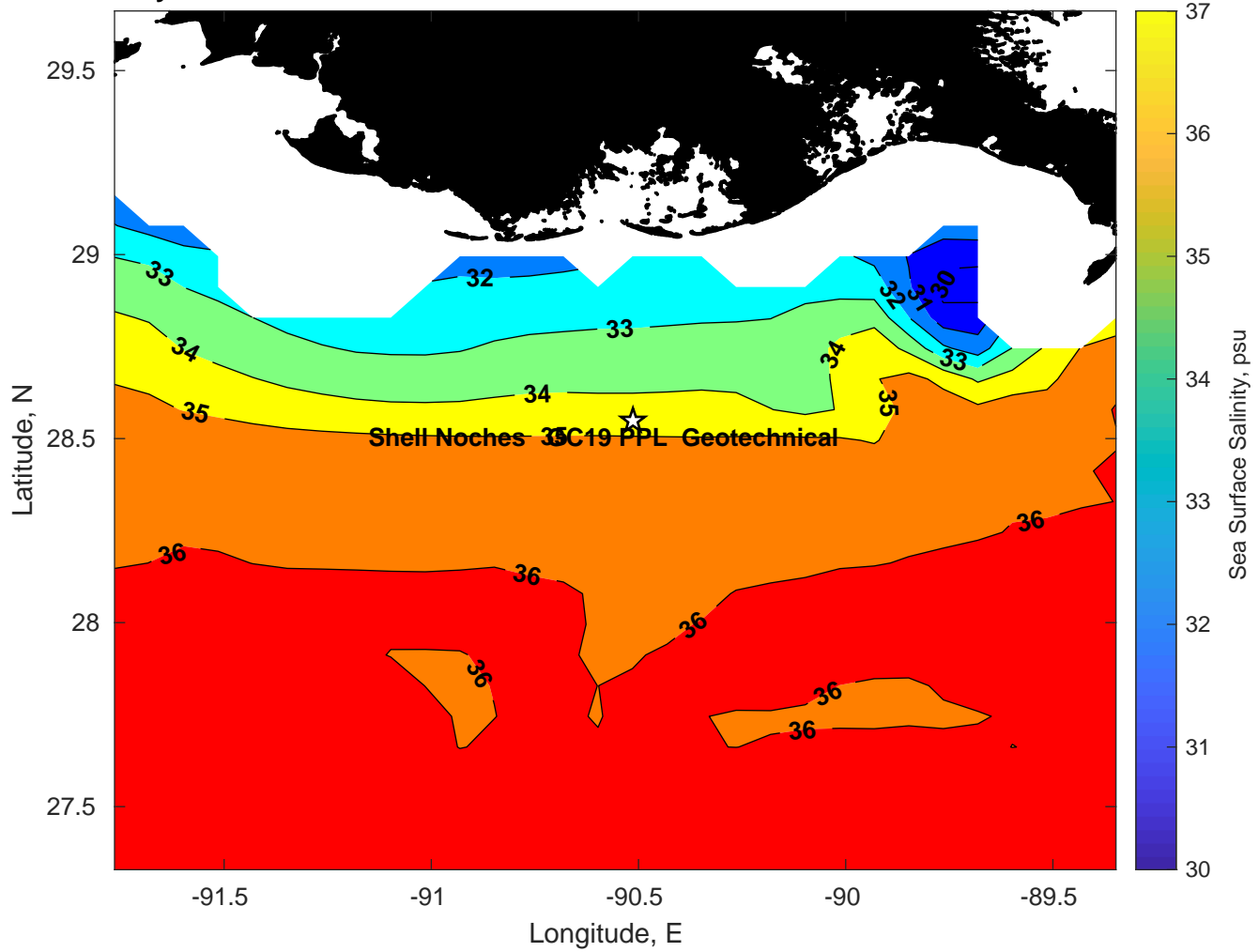
Surface Salinity for Shell Noches GC19 PPL Geotechnical at 03-Mar-2025 00:00:00
