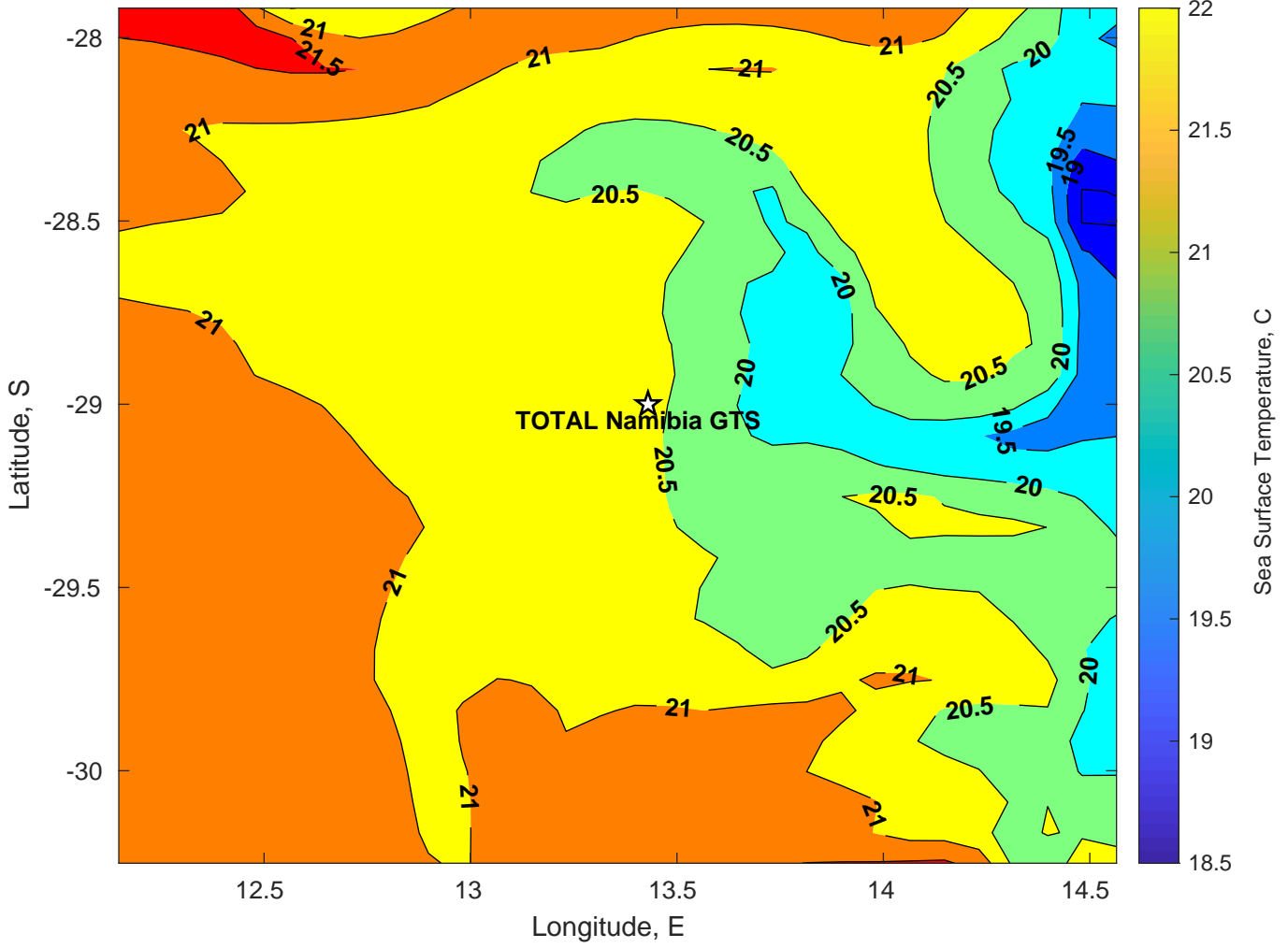
SST for TOTAL Namibia GTS at 03-Mar-2025 00:00:00
