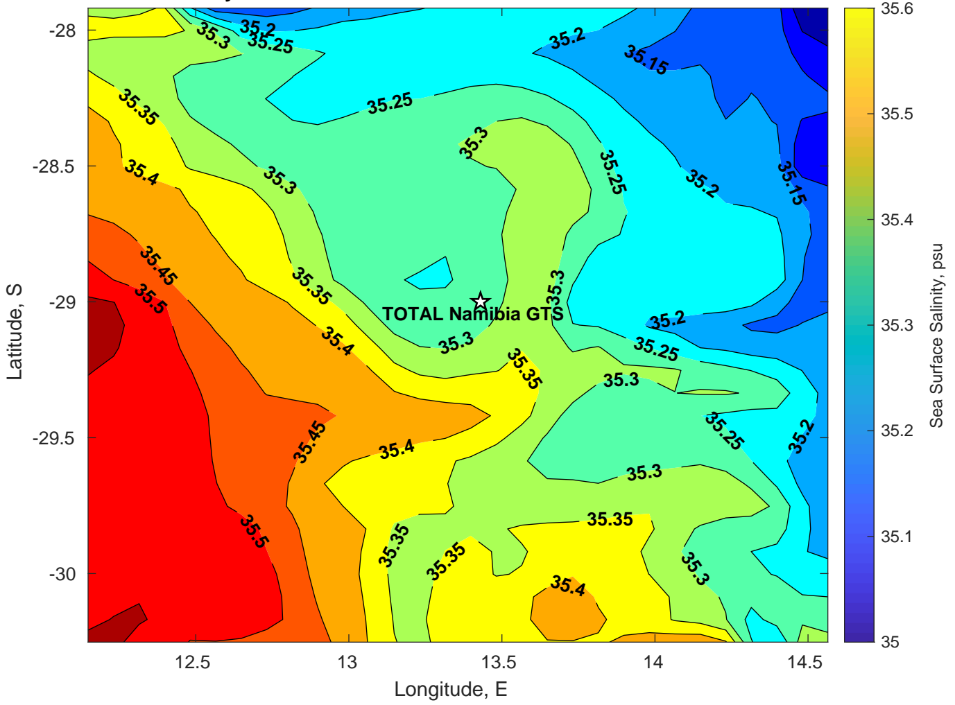
Surface Salinity for TOTAL Namibia GTS at 03-Mar-2025 00:00:00
