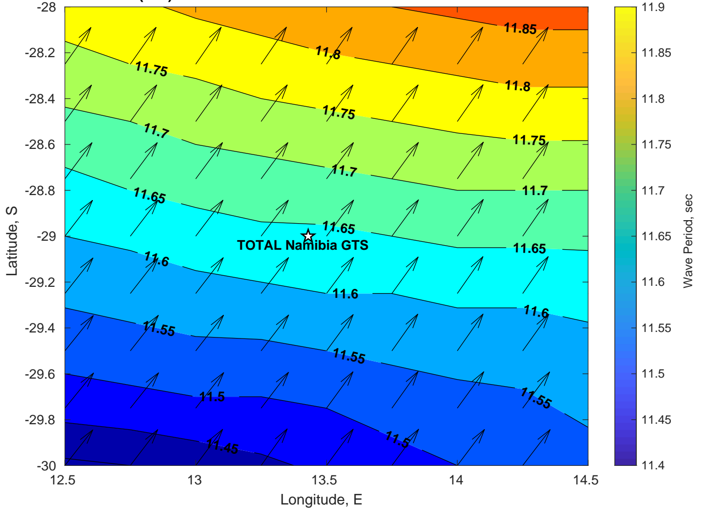
Wave Period (sec) for TOTAL Namibia GTS at 04-Mar-2025 09:00:00
