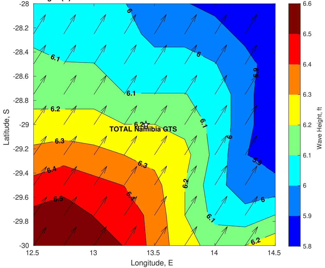
Wave Height (ft) for TOTAL Namibia GTS at 04-Mar-2025 09:00:00
