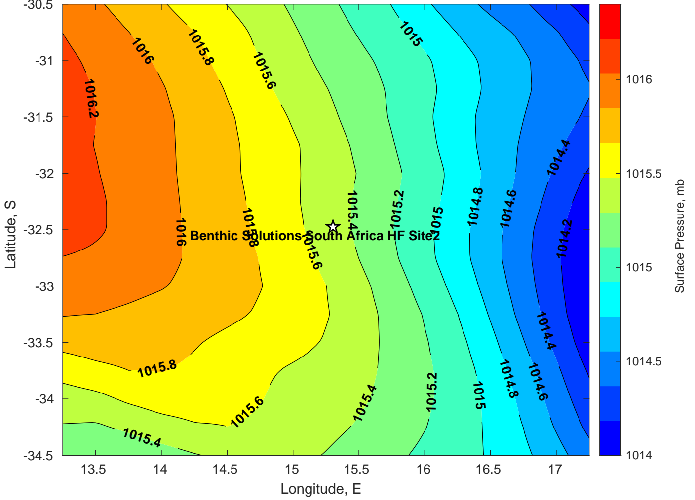
Surface Pressure (mb) for Benthic Solutions South Africa HF Site2 at 06-Mar-2025 00:00:00
