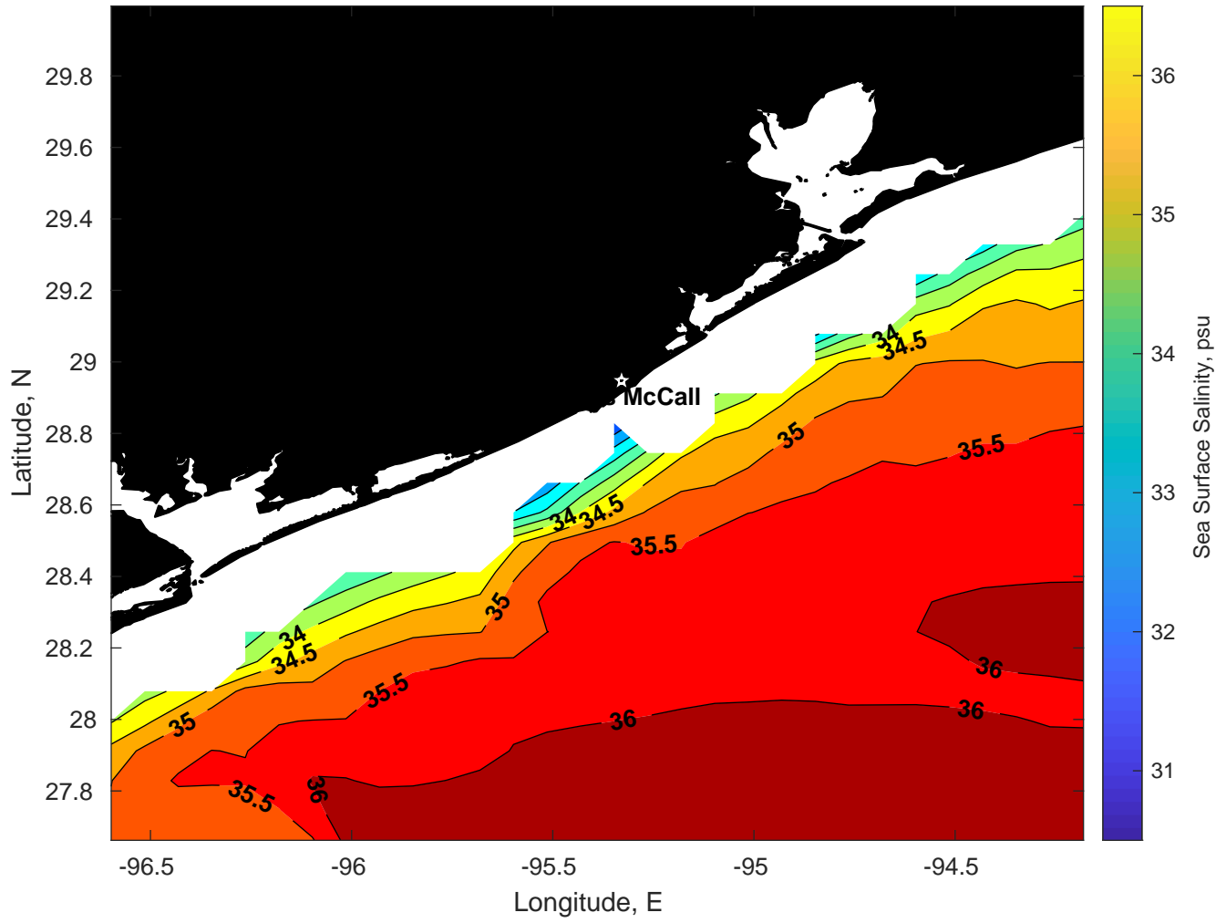
Surface Salinity for Brooks McCall at 04-Mar-2025 00:00:00
