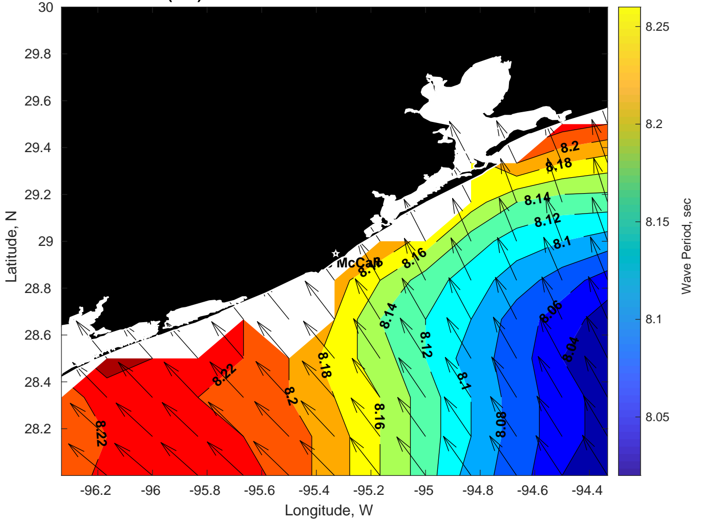
Wave Period (sec) for Brooks McCall at 05-Mar-2025 09:00:00
