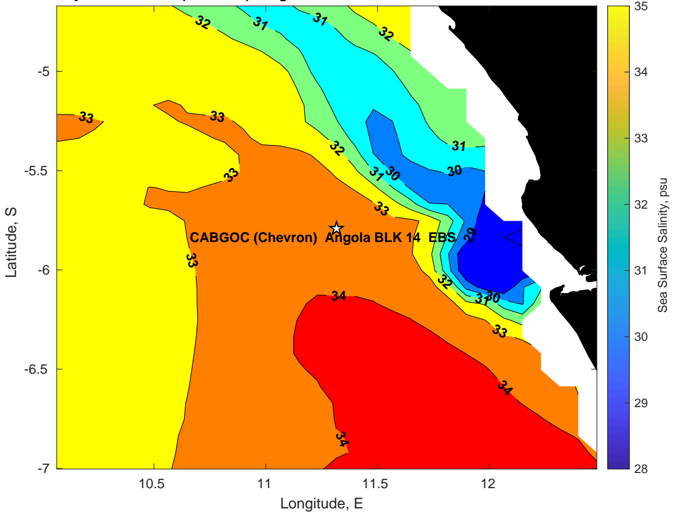
Surface Salinity for CABGOC (Chevron) Angola BLK 14 EBS at 04-Mar-2025 00:00:00
