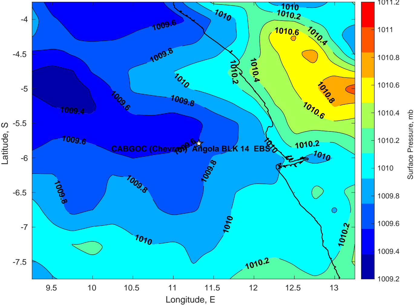
Surface Pressure (mb) for CABGOC (Chevron) Angola BLK 14 EBS at 06-Mar-2025 00:00:00
