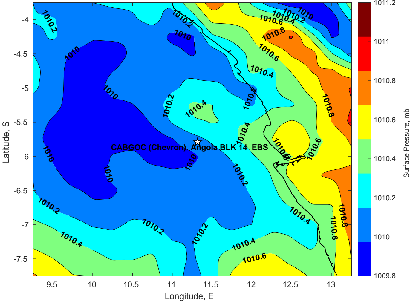
Surface Pressure (mb) for CABGOC (Chevron) Angola BLK 14 EBS at 07-Mar-2025 00:00:00
