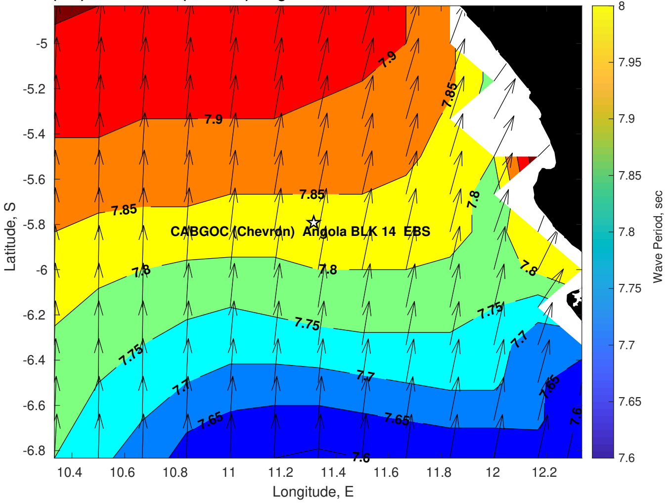
Wave Period (sec) for CABGOC (Chevron) Angola BLK 14 EBS at 05-Mar-2025 09:00:00
