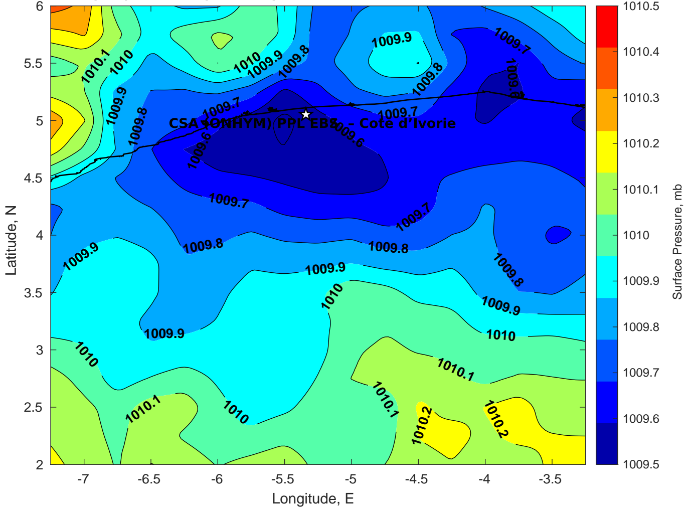
Surface Pressure (mb) for CSA (ONHYM) PPL EBS - Cote d'Ivoire at 06-Mar-2025 06:00:00
