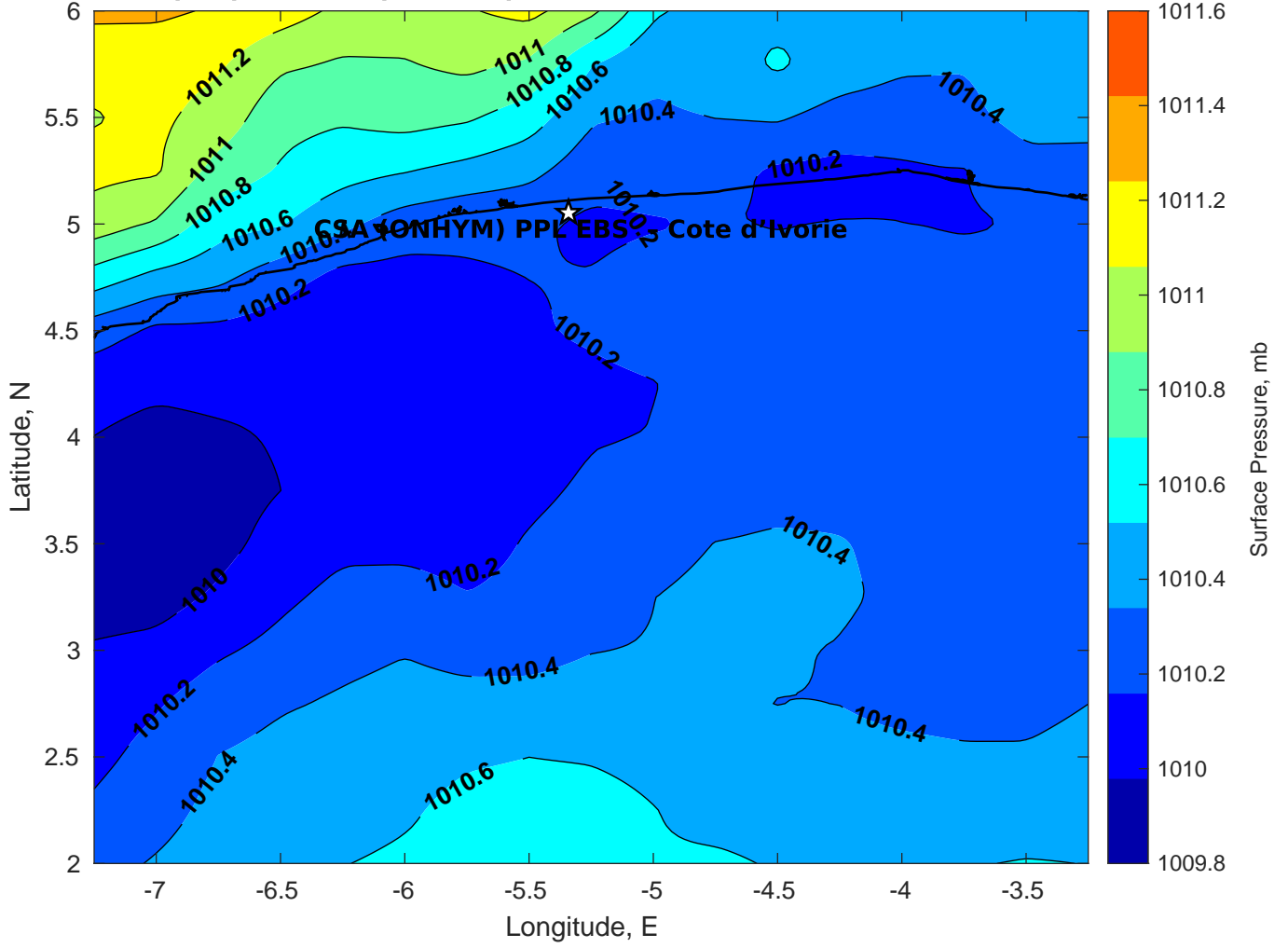
Surface Pressure (mb) for CSA (ONHYM) PPL EBS - Cote d'Ivoire at 07-Mar-2025 06:00:00
