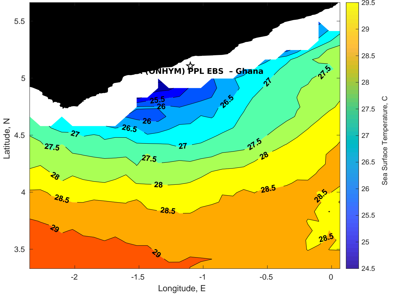
SST for CSA (ONHYM) PPL EBS - Ghana at 04-Mar-2025 00:00:00
