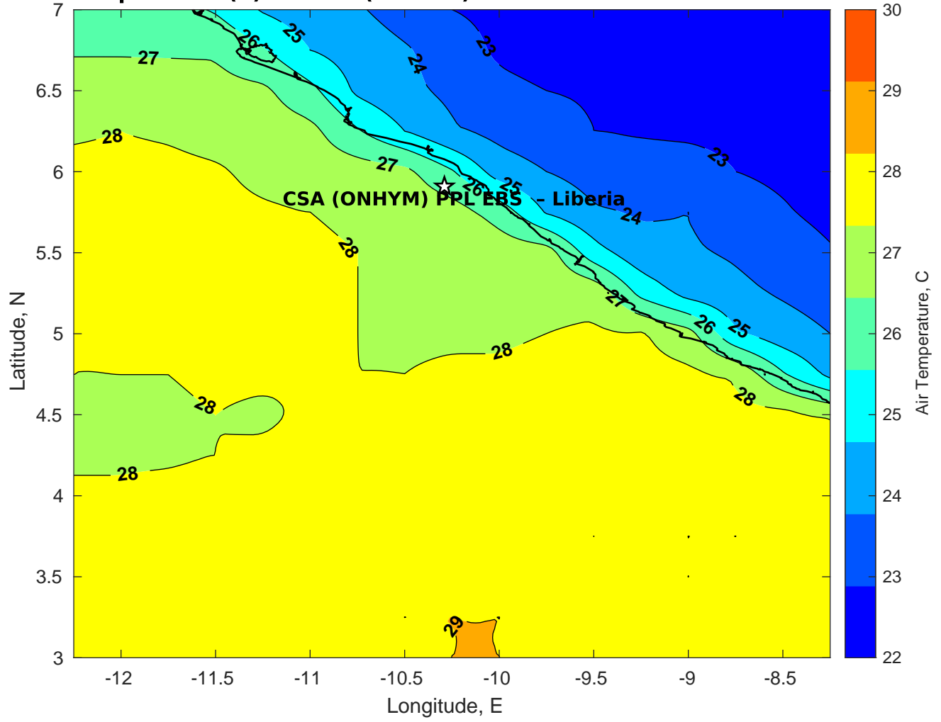
Air Temperature (C) for CSA (ONHYM) PPL EBS - Liberia at 05-Mar-2025
