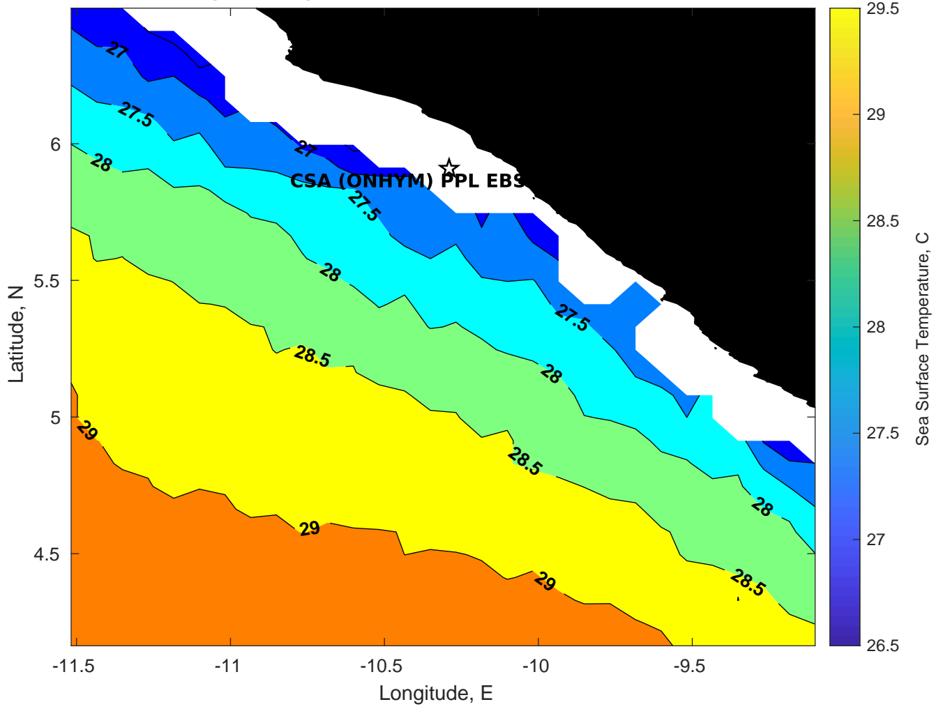
SST for CSA (ONHYM) PPL EBS - Liberia at 04-Mar-2025 00:00:00
