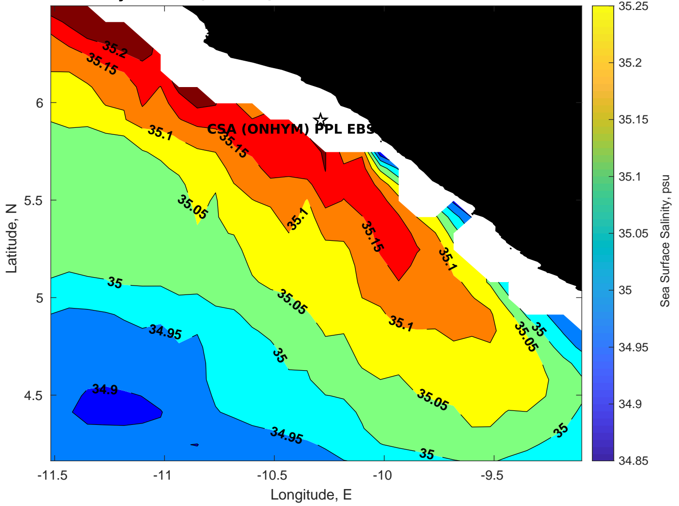
Surface Salinity for CSA (ONHYM) PPL EBS - Liberia at 04-Mar-2025 00:00:00
