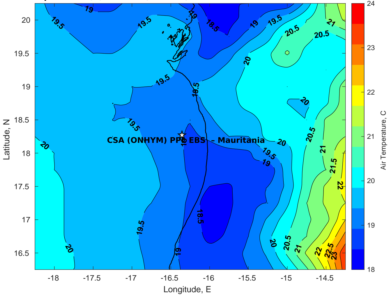
Air Temperature (C) for CSA (ONHYM) PPL EBS - Mauritania at 05-Mar-2025
