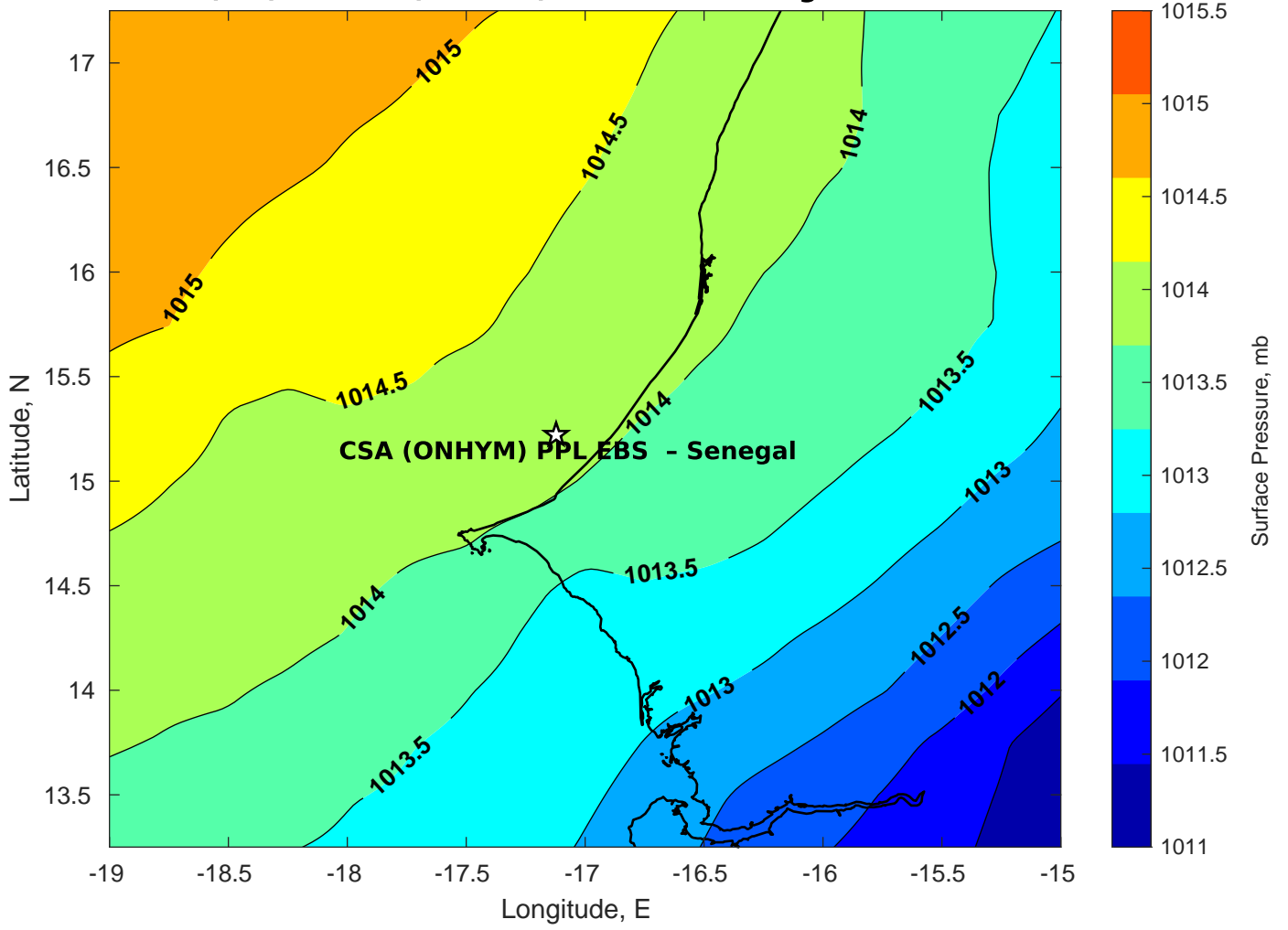
Surface Pressure (mb) for CSA (ONHYM) PPL EBS - Senegal at 06-Mar-2025 00:00:00
