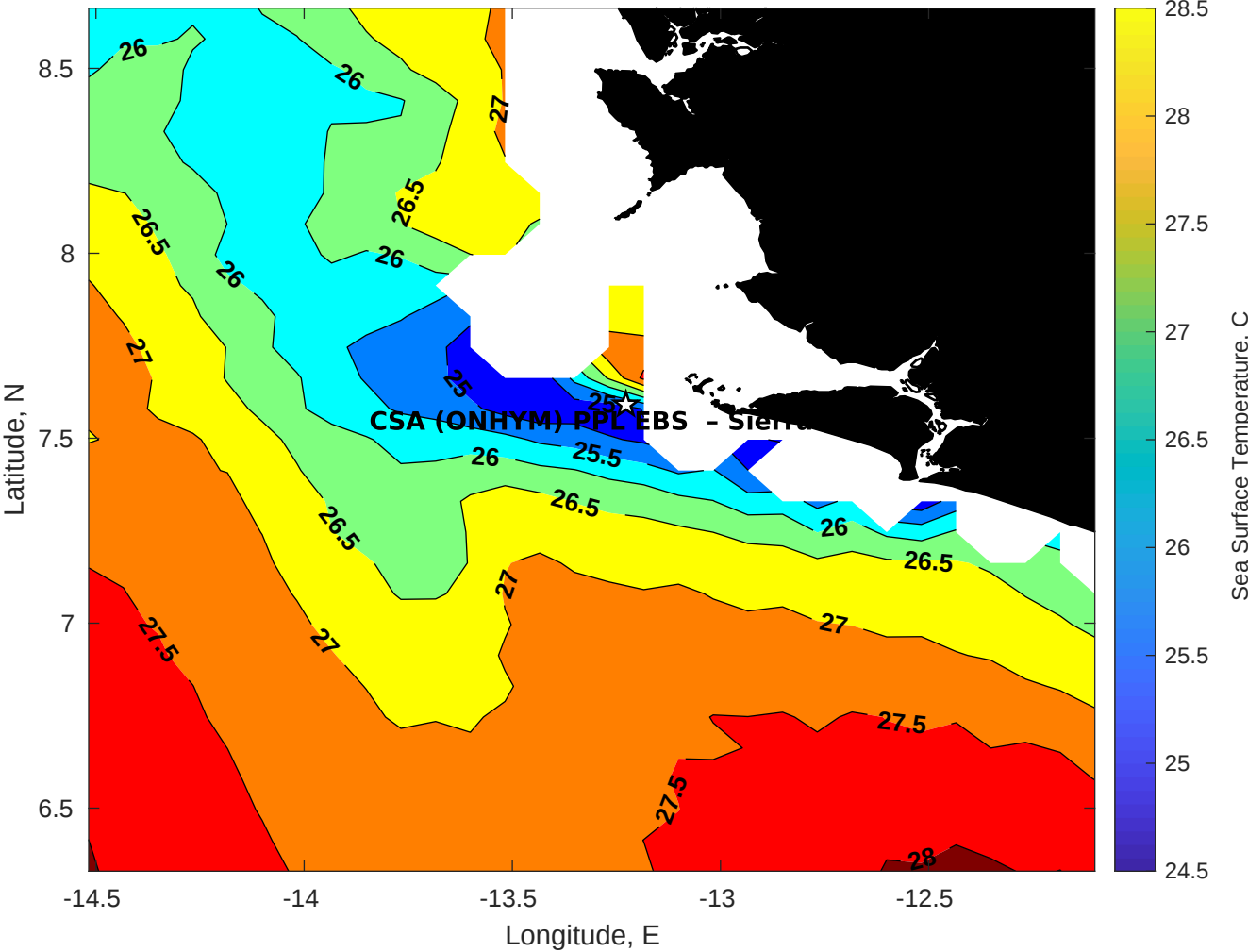
SST for CSA (ONHYM) PPL EBS - Sierra Leone at 04-Mar-2025 00:00:00
