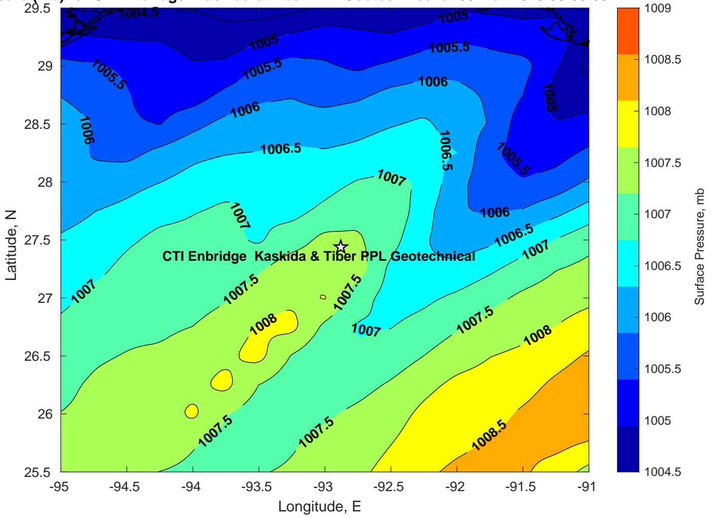
Surface Pressure (mb) for CTI Enbridge Kaskida & Tiber PPL Geotechnical at 05-Mar-2025 00:00:00
