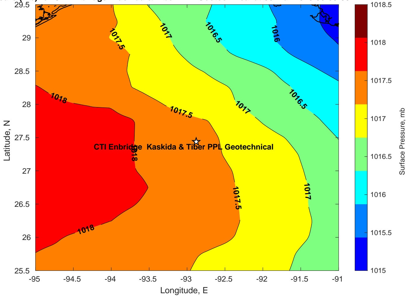
Surface Pressure (mb) for CTI Enbridge Kaskida & Tiber PPL Geotechnical at 06-Mar-2025 00:00:00
