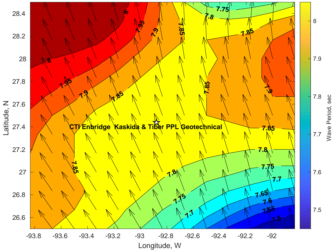
Wave Period (sec) for CTI Enbridge Kaskida & Tiber PPL Geotechnical at 05-Mar-2025 09:00:00
