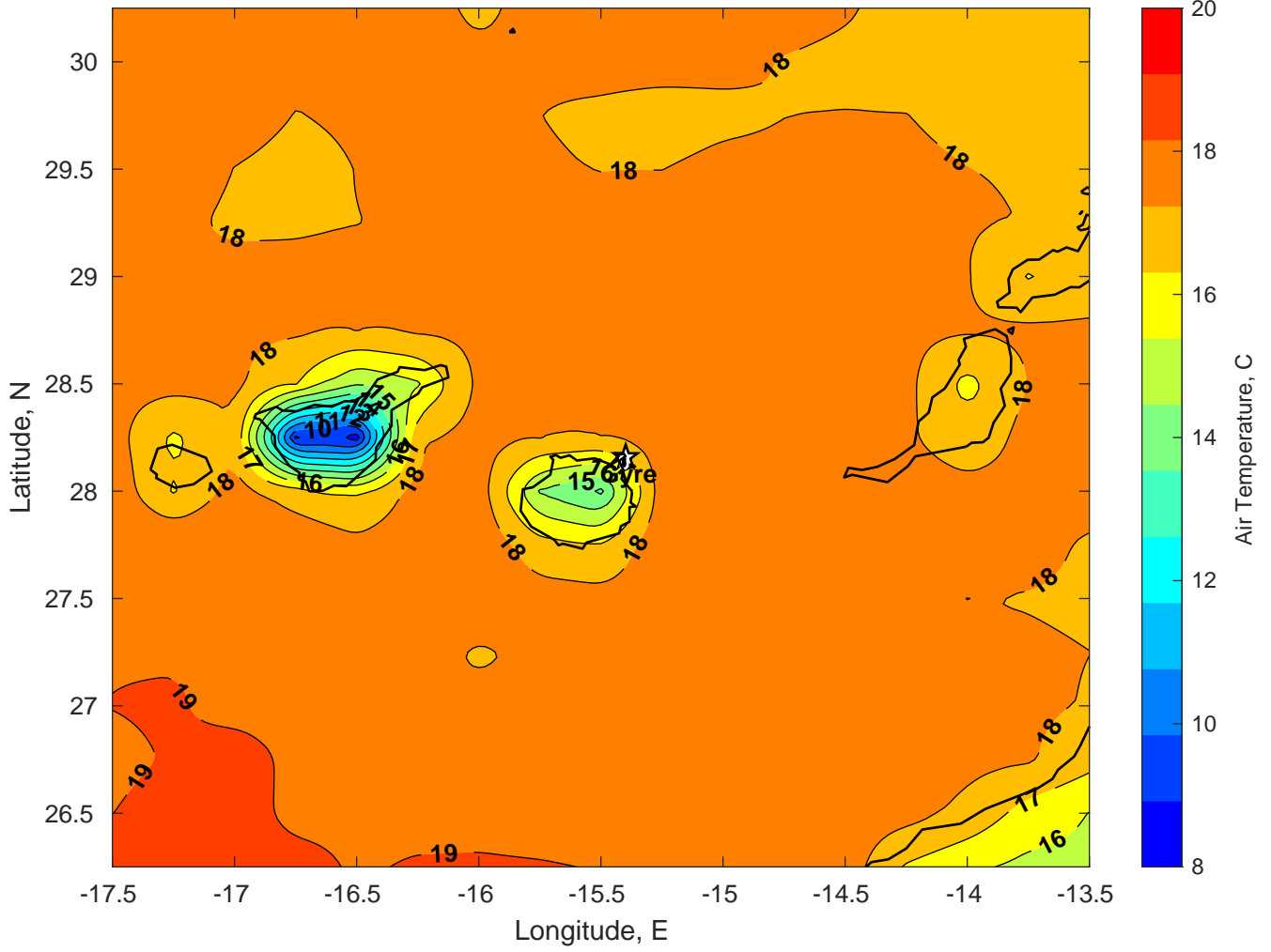
Air Temperature (C) for Gyre at 05-Mar-2025
