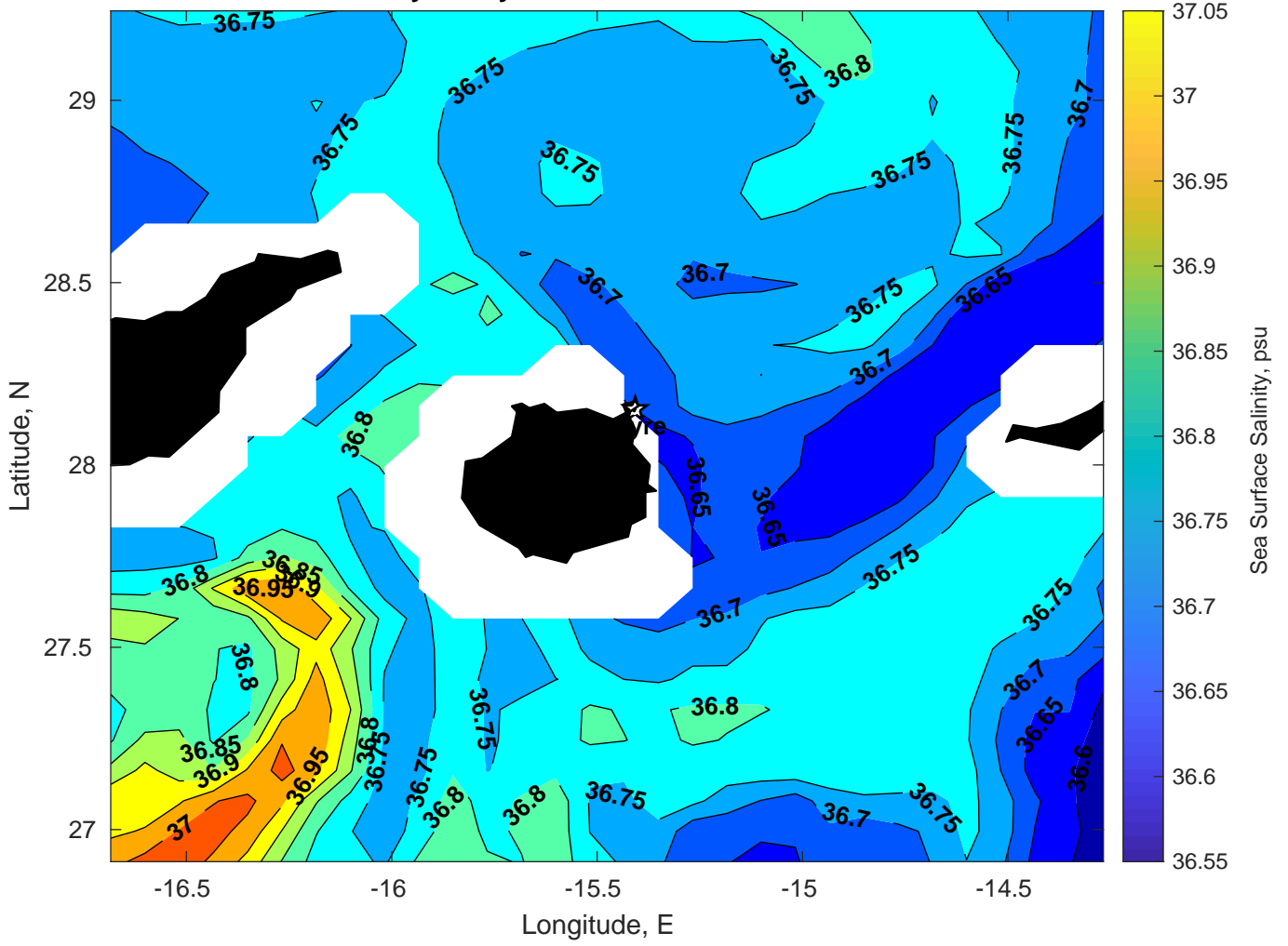
Surface Salinity for Gyre at 04-Mar-2025 00:00:00
