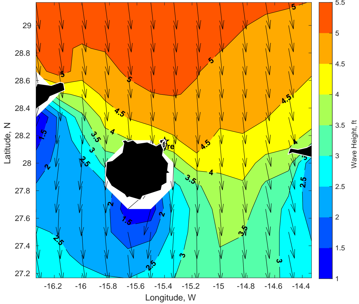
Wave Height (ft) for Gyre at 05-Mar-2025 09:00:00
