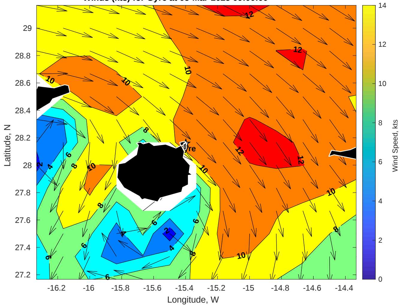
Winds (kts) for Gyre at 05-Mar-2025 09:00:00
