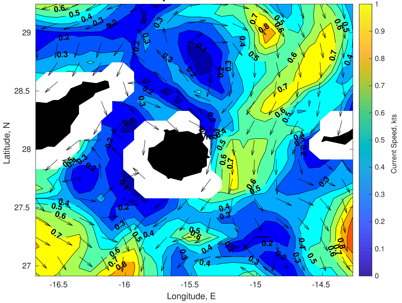
Surface Currents for Gyre at 04-Mar-2025 00:00:00
