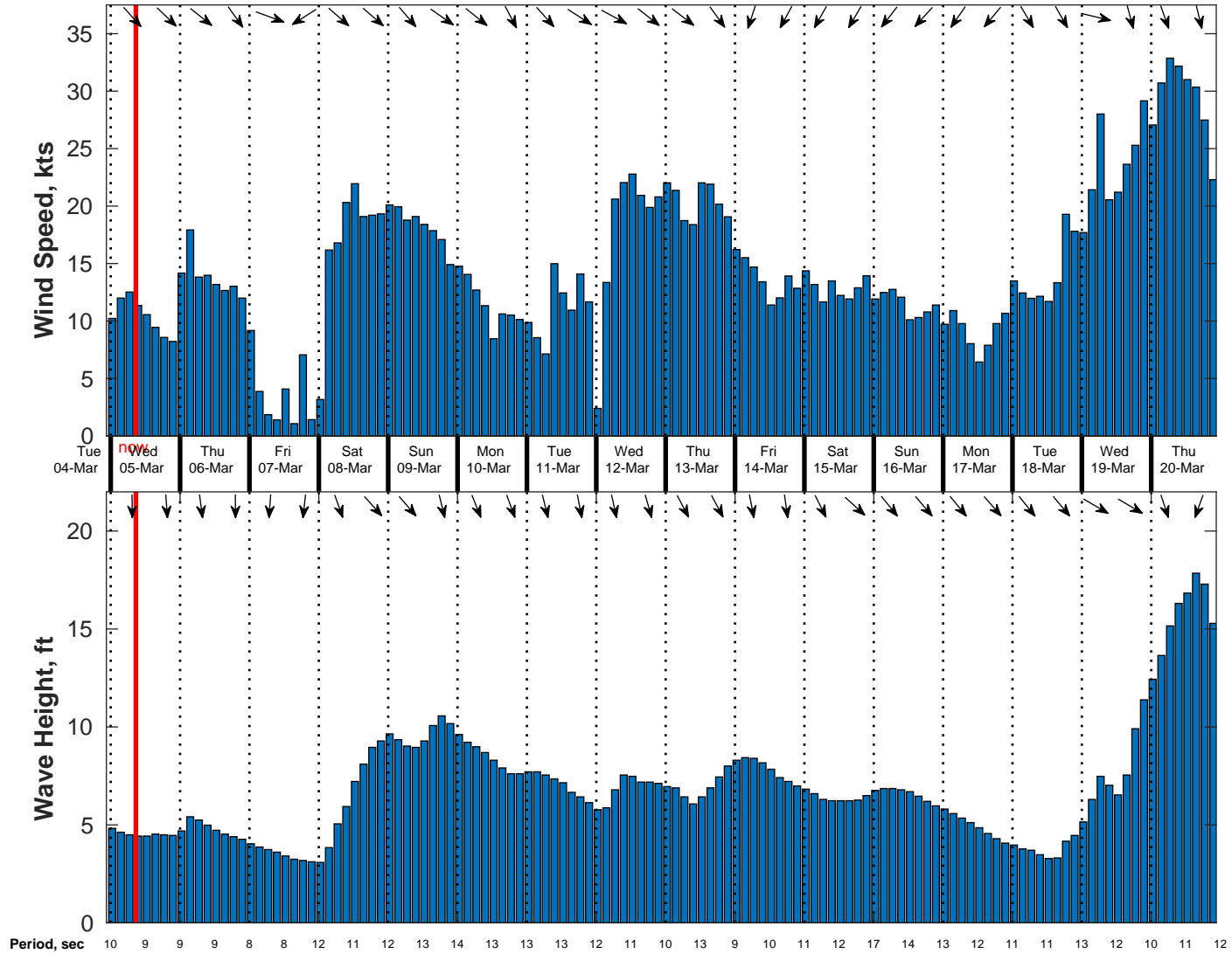
Wind & Wave Forecast for Gyre from 04-Mar-2025 23:00:00 to 20-Mar-2025 23:00:00
