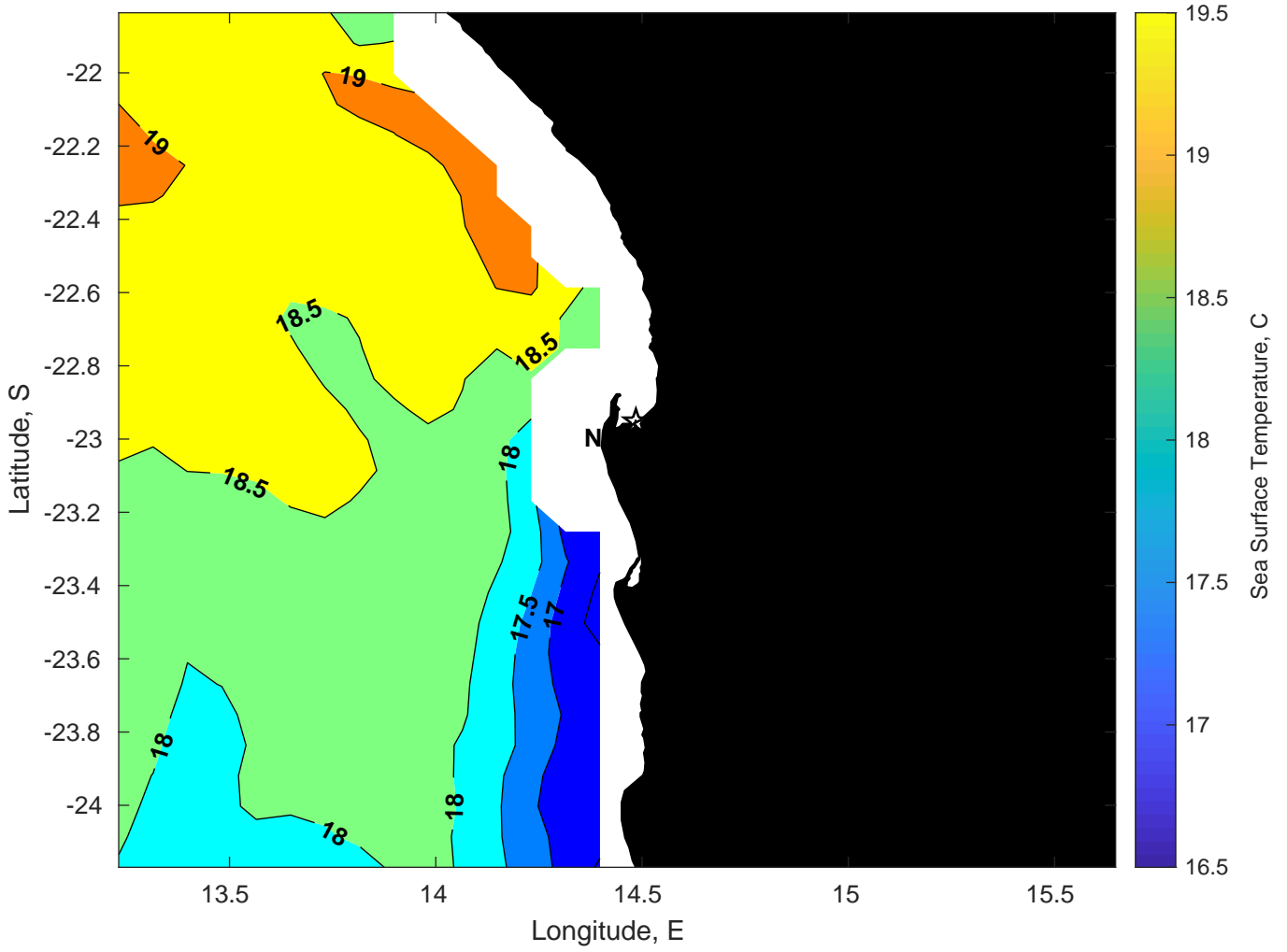
SST for Nautilus at 04-Mar-2025 00:00:00
