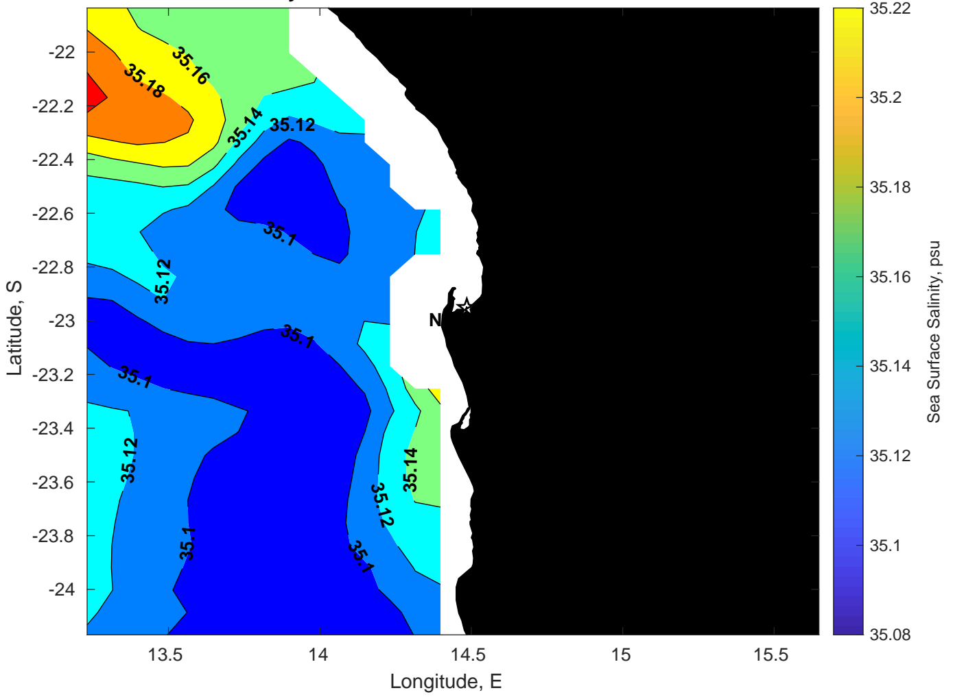
Surface Salinity for Nautilus at 04-Mar-2025 00:00:00
