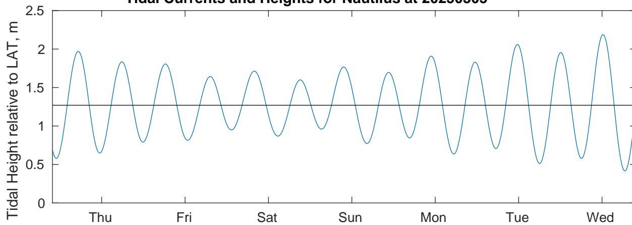
Tidal Currents and Heights for Nautilus at 20250305
